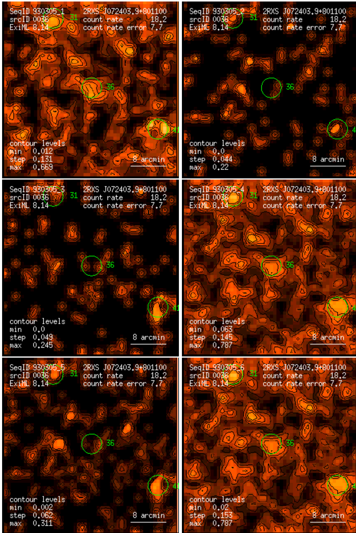
Figure 36: RASS 930305: detection 0036: band rate images, Gaussian filter: (1) PSPC channels 11 – 41, (2) 52 – 90, (3) 91 – 201, (4) 11 – 235, (5) 52 – 201, (6) 11 – 201. Broad band rates in counts/ks. Band rate contour levels in counts/ks/arcmin 2 .
