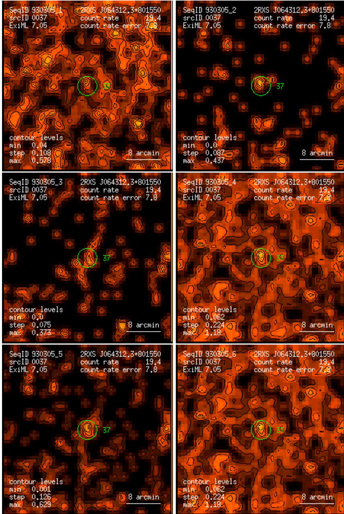
Figure 37: RASS 930305: detection 0037: band rate images, Gaussian filter: (1) PSPC channels 11 – 41, (2) 52 – 90, (3) 91 – 201, (4) 11 – 235, (5) 52 – 201, (6) 11 – 201. Broad band rates in counts/ks. Band rate contour levels in counts/ks/arcmin 2 .
