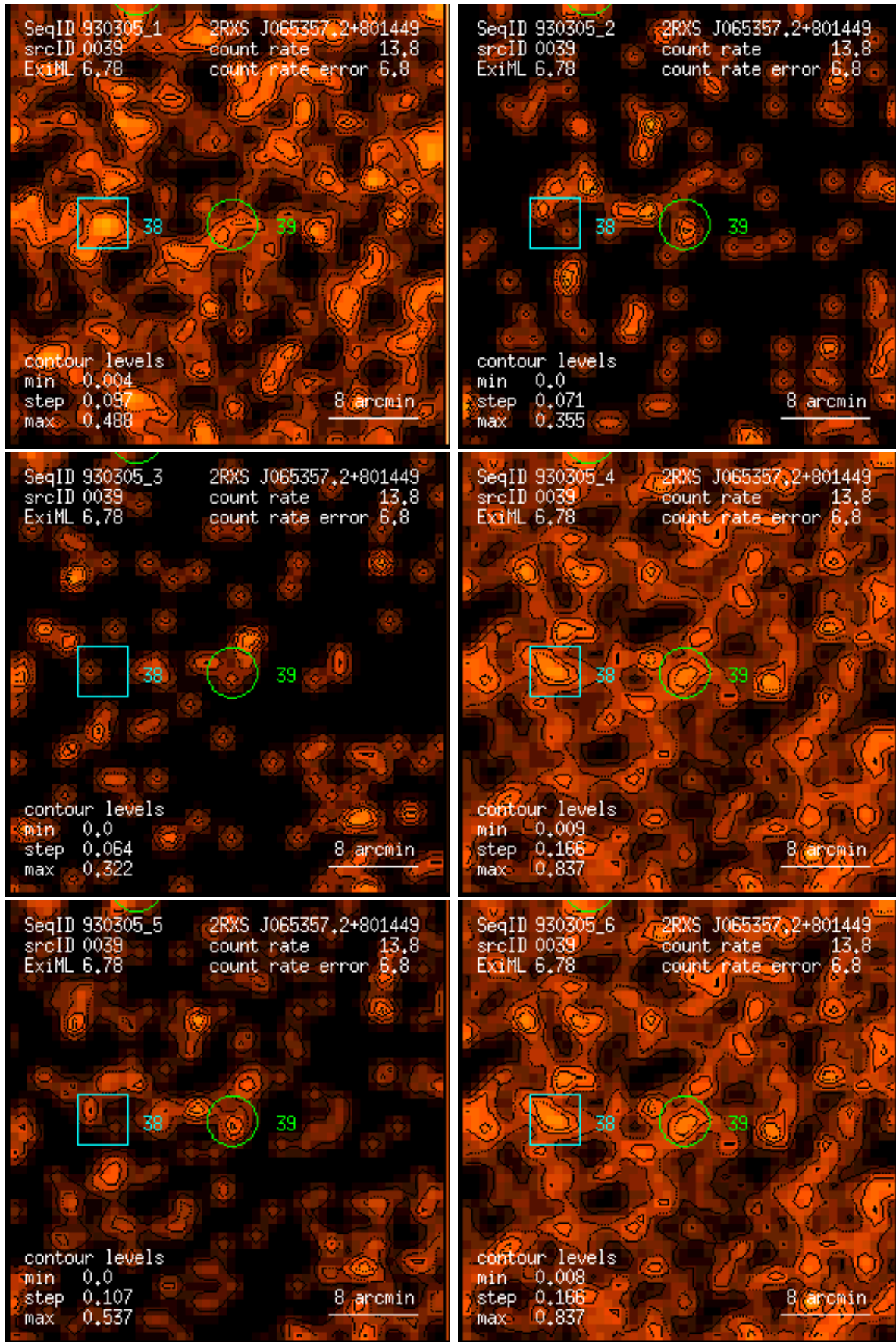
Figure 39: RASS 930305: detection 0039: band rate images, Gaussian filter: (1) PSPC channels 11 – 41, (2) 52 – 90, (3) 91 – 201, (4) 11 – 235, (5) 52 – 201, (6) 11 – 201. Broad band rates in counts/ks. Band rate contour levels in counts/ks/arcmin 2 .
