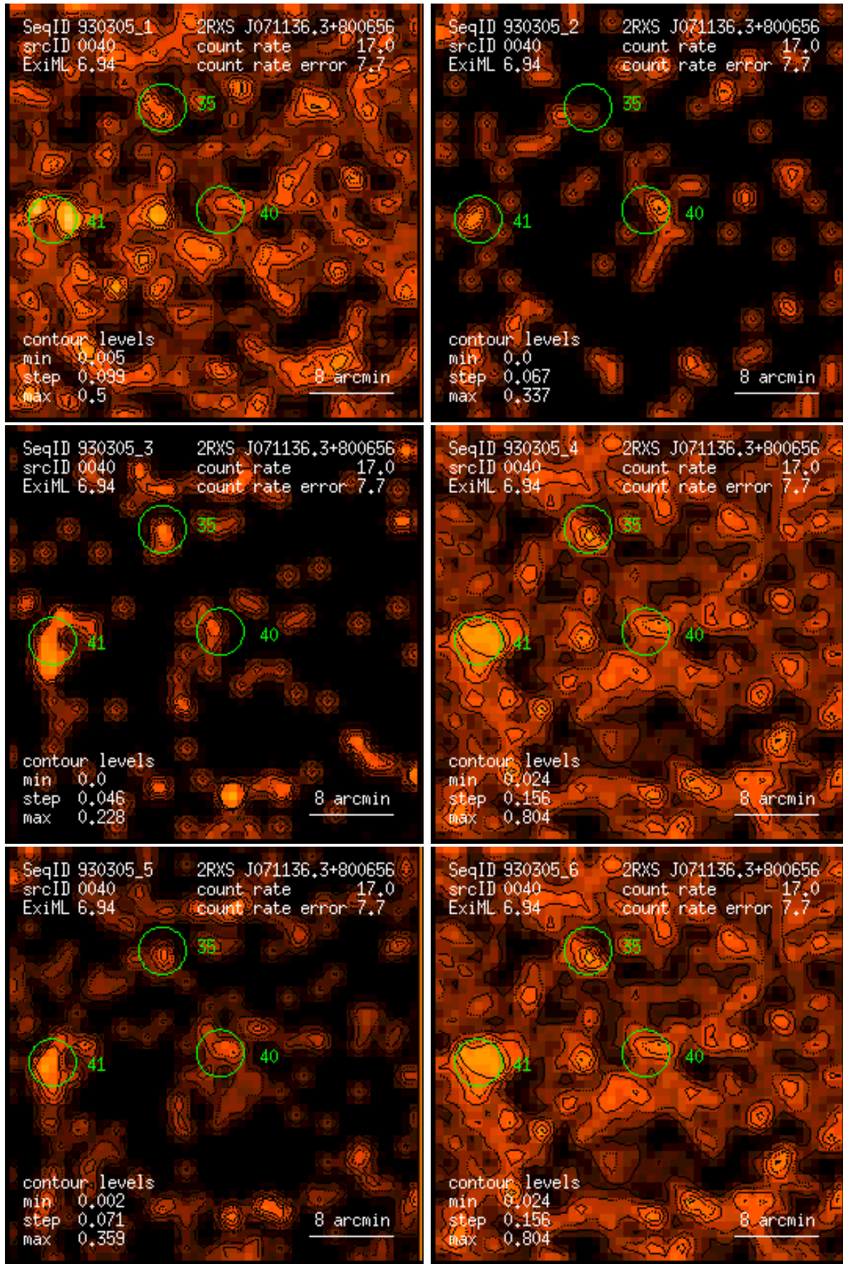
Figure 40: RASS 930305: detection 0040: band rate images, Gaussian filter: (1) PSPC channels 11 – 41, (2) 52 – 90, (3) 91 – 201, (4) 11 – 235, (5) 52 – 201, (6) 11 – 201. Broad band rates in counts/ks. Band rate contour levels in counts/ks/arcmin 2 .
