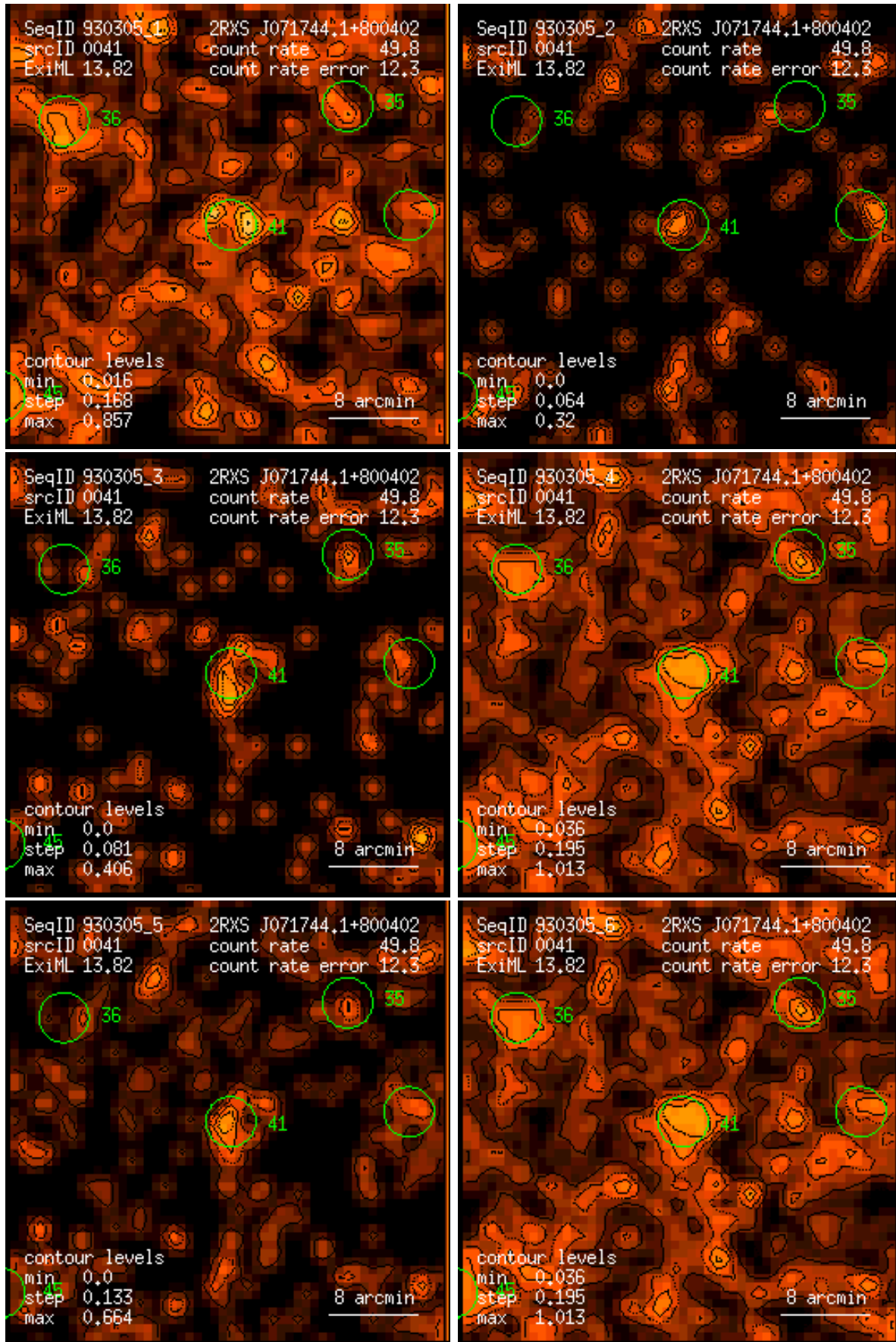
Figure 41: RASS 930305: detection 0041: band rate images, Gaussian filter: (1) PSPC channels 11 – 41, (2) 52 – 90, (3) 91 – 201, (4) 11 – 235, (5) 52 – 201, (6) 11 – 201. Broad band rates in counts/ks. Band rate contour levels in counts/ks/arcmin 2 .
