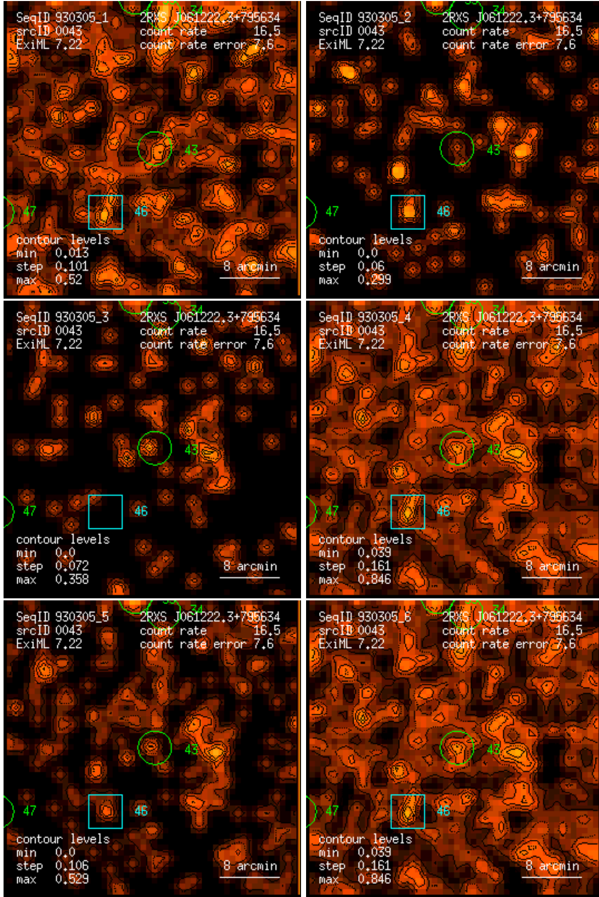
Figure 43: RASS 930305: detection 0043: band rate images, Gaussian filter: (1) PSPC channels 11 – 41, (2) 52 – 90, (3) 91 – 201, (4) 11 – 235, (5) 52 – 201, (6) 11 – 201. Broad band rates in counts/ks. Band rate contour levels in counts/ks/arcmin 2 .
