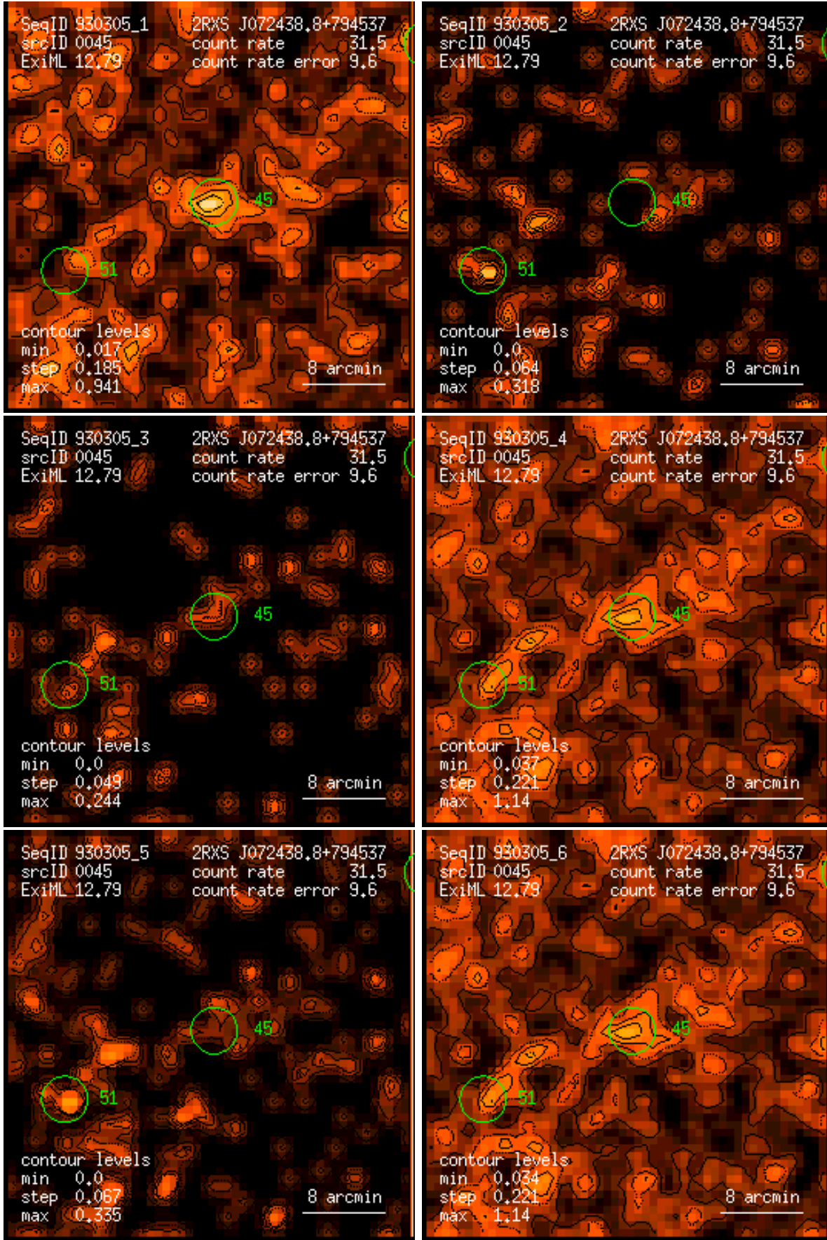
Figure 45: RASS 930305: detection 0045: band rate images, Gaussian filter: (1) PSPC channels 11 – 41, (2) 52 – 90, (3) 91 – 201, (4) 11 – 235, (5) 52 – 201, (6) 11 – 201. Broad band rates in counts/ks. Band rate contour levels in counts/ks/arcmin 2 .
