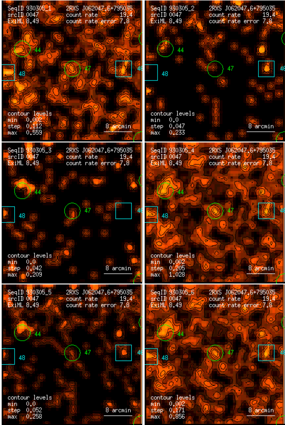
Figure 47: RASS 930305: detection 0047: band rate images, Gaussian filter: (1) PSPC channels 11 – 41, (2) 52 – 90, (3) 91 – 201, (4) 11 – 235, (5) 52 – 201, (6) 11 – 201. Broad band rates in counts/ks. Band rate contour levels in counts/ks/arcmin 2 .
