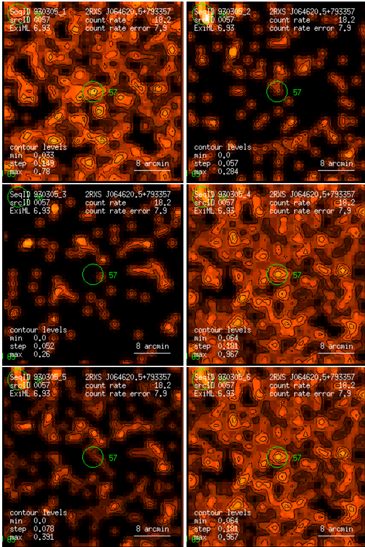
Figure 57: RASS 930305: detection 0057: band rate images, Gaussian filter: (1) PSPC channels 11 – 41, (2) 52 – 90, (3) 91 – 201, (4) 11 – 235, (5) 52 – 201, (6) 11 – 201. Broad band rates in counts/ks. Band rate contour levels in counts/ks/arcmin 2 .
