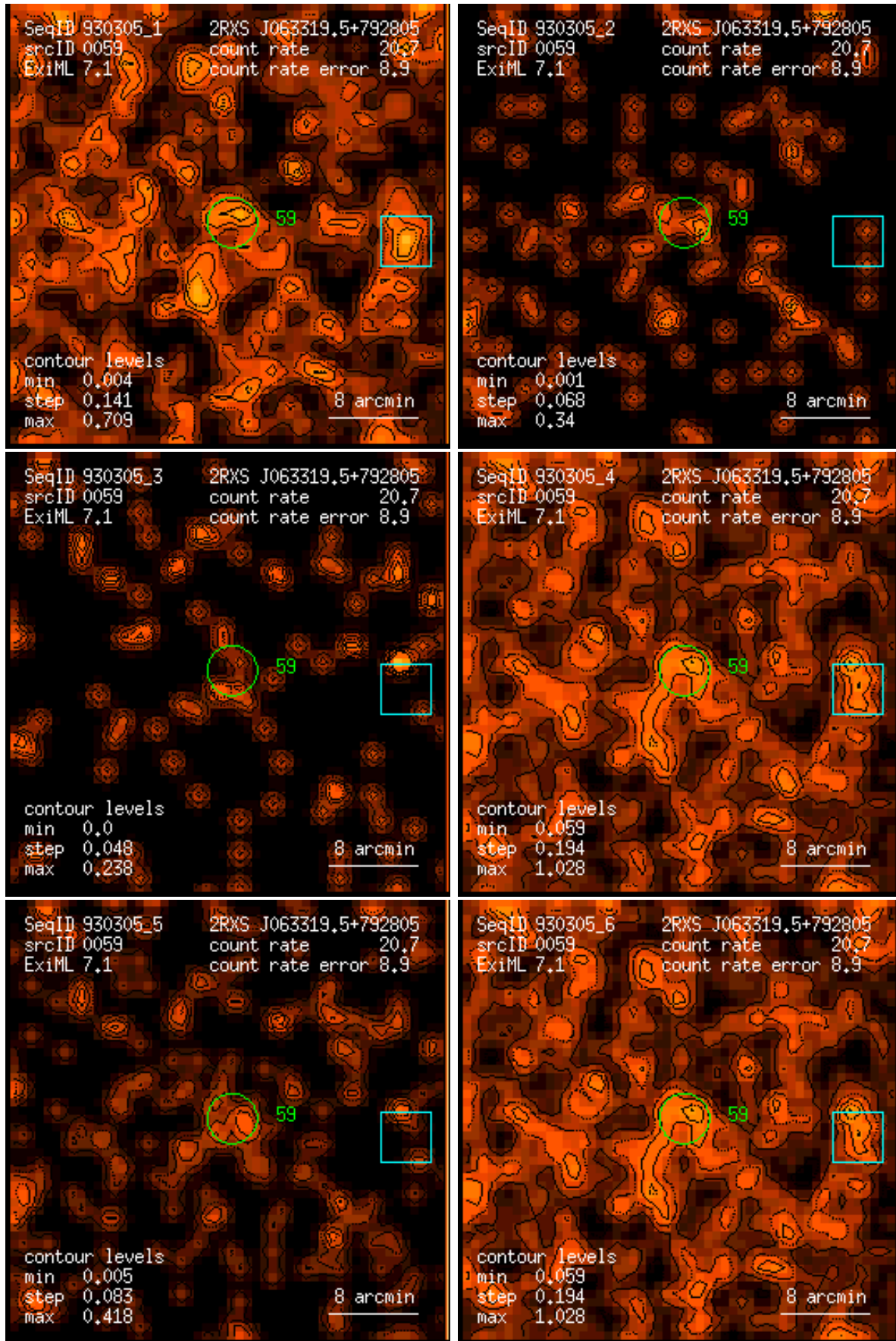
Figure 59: RASS 930305: detection 0059: band rate images, Gaussian filter: (1) PSPC channels 11 – 41, (2) 52 – 90, (3) 91 – 201, (4) 11 – 235, (5) 52 – 201, (6) 11 – 201. Broad band rates in counts/ks. Band rate contour levels in counts/ks/arcmin 2 .
