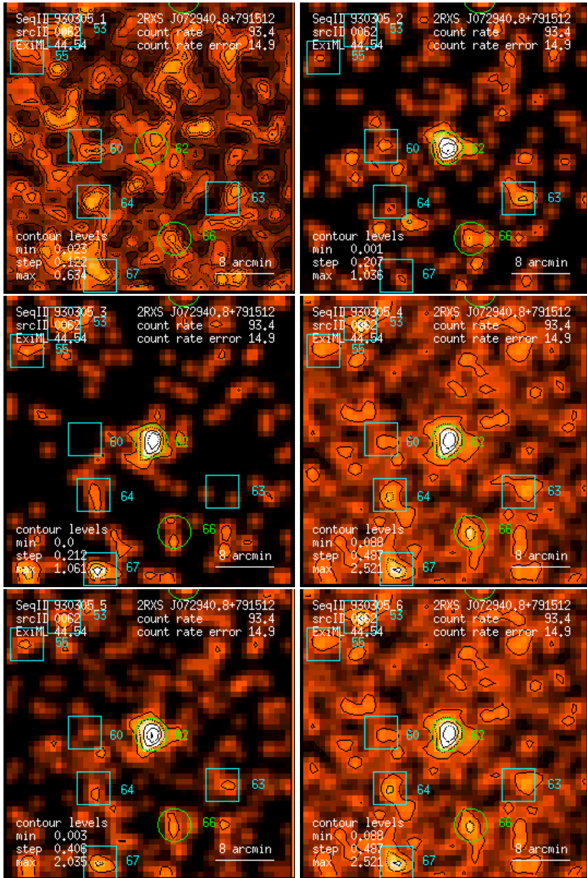
Figure 62: RASS 930305: detection 0062: band rate images, Gaussian filter: (1) PSPC channels 11 – 41, (2) 52 – 90, (3) 91 – 201, (4) 11 – 235, (5) 52 – 201, (6) 11 – 201. Broad band rates in counts/ks. Band rate contour levels in counts/ks/arcmin 2 .
