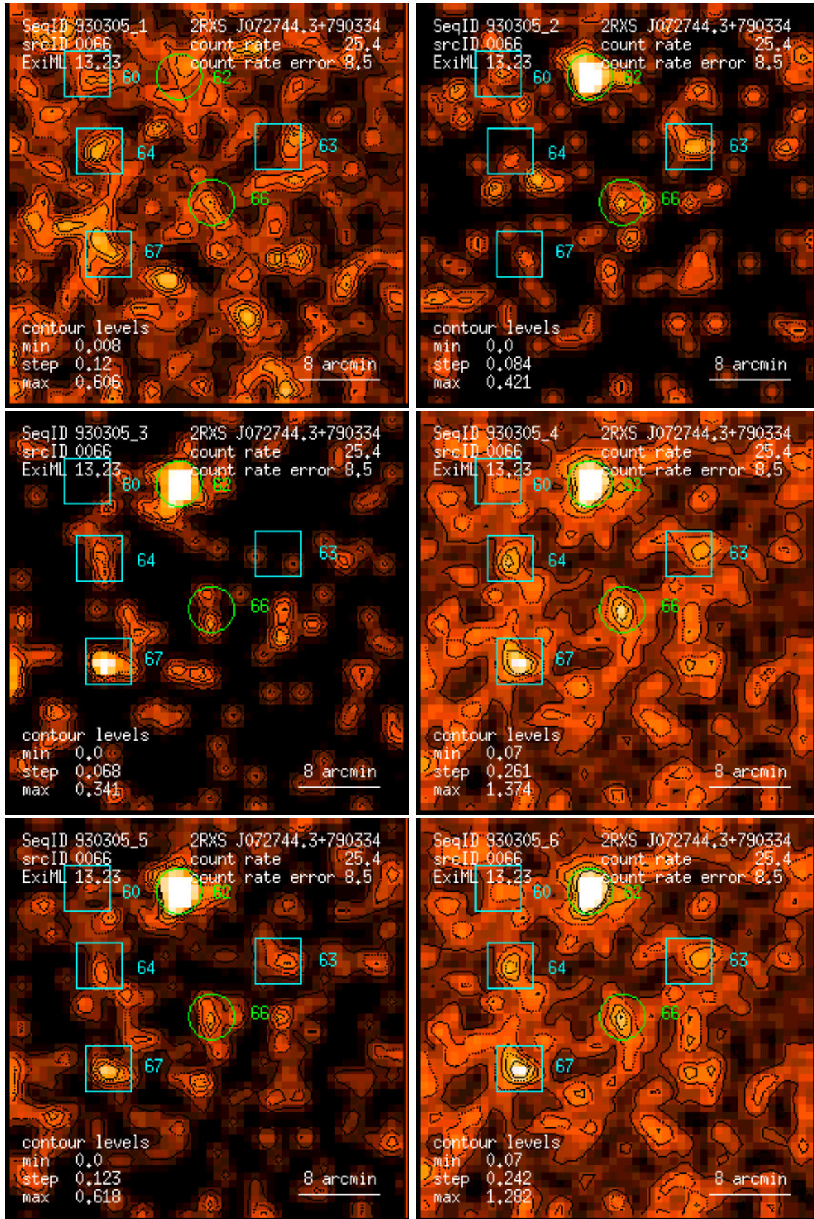
Figure 66: RASS 930305: detection 0066: band rate images, Gaussian filter: (1) PSPC channels 11 – 41, (2) 52 – 90, (3) 91 – 201, (4) 11 – 235, (5) 52 – 201, (6) 11 – 201. Broad band rates in counts/ks. Band rate contour levels in counts/ks/arcmin 2 .
