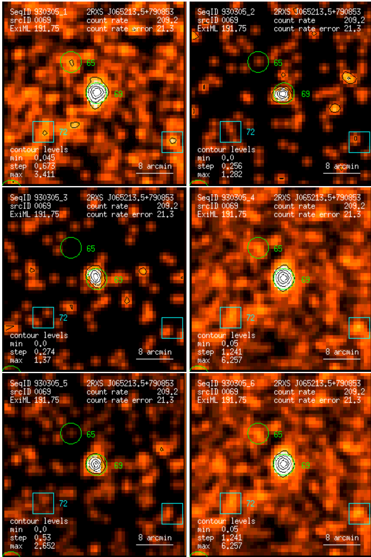
Figure 69: RASS 930305: detection 0069: band rate images, Gaussian filter: (1) PSPC channels 11 – 41, (2) 52 – 90, (3) 91 – 201, (4) 11 – 235, (5) 52 – 201, (6) 11 – 201. Broad band rates in counts/ks. Band rate contour levels in counts/ks/arcmin 2 .
