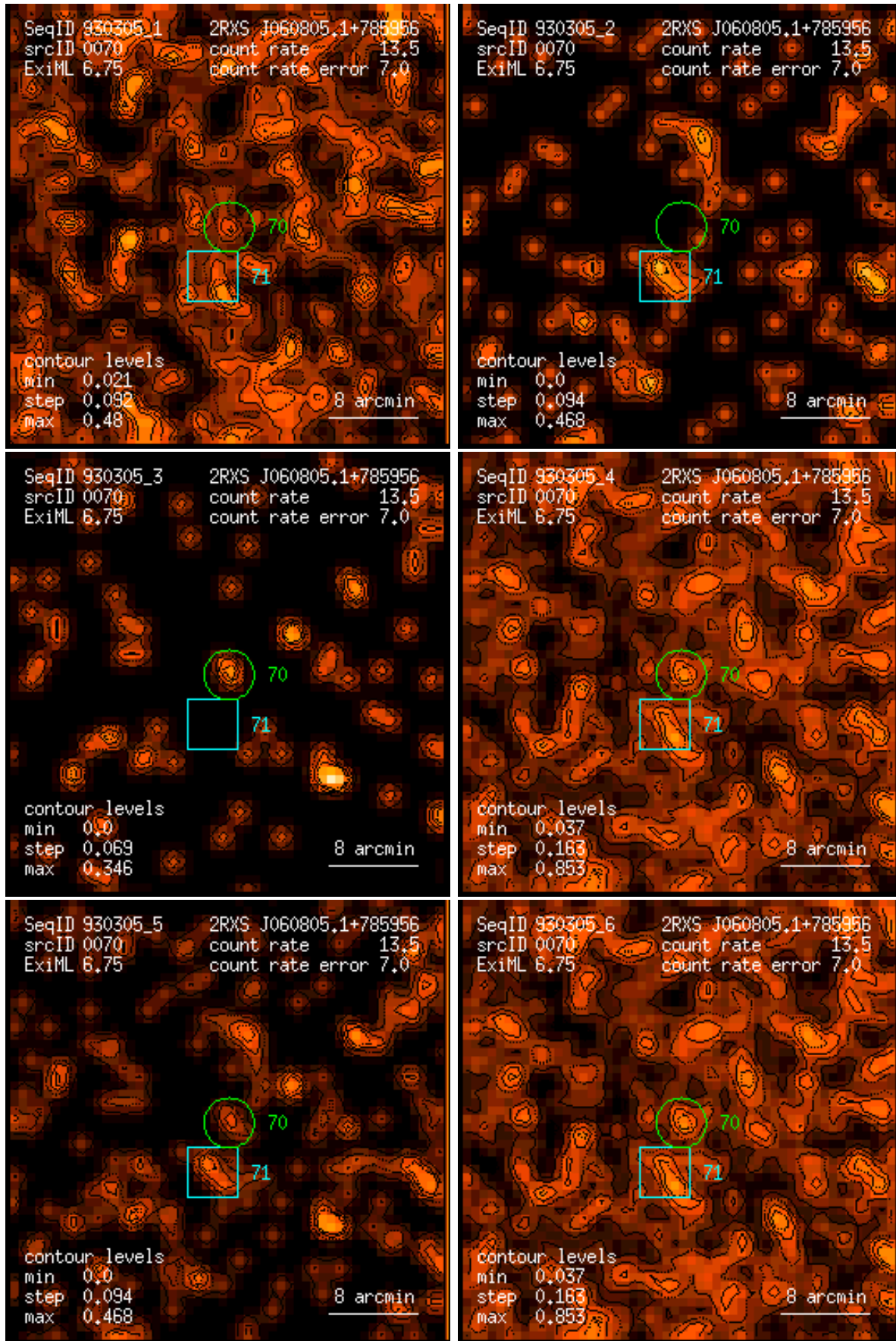
Figure 70: RASS 930305: detection 0070: band rate images, Gaussian filter: (1) PSPC channels 11 – 41, (2) 52 – 90, (3) 91 – 201, (4) 11 – 235, (5) 52 – 201, (6) 11 – 201. Broad band rates in counts/ks. Band rate contour levels in counts/ks/arcmin 2 .
