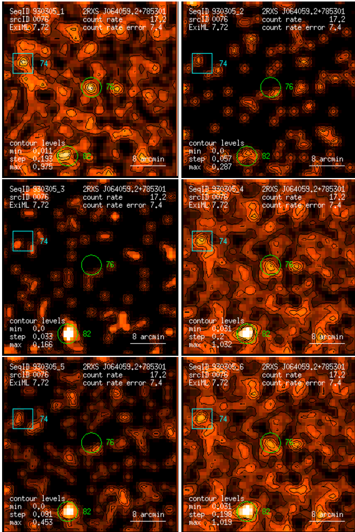
Figure 76: RASS 930305: detection 0076: band rate images, Gaussian filter: (1) PSPC channels 11 – 41, (2) 52 – 90, (3) 91 – 201, (4) 11 – 235, (5) 52 – 201, (6) 11 – 201. Broad band rates in counts/ks. Band rate contour levels in counts/ks/arcmin 2 .
