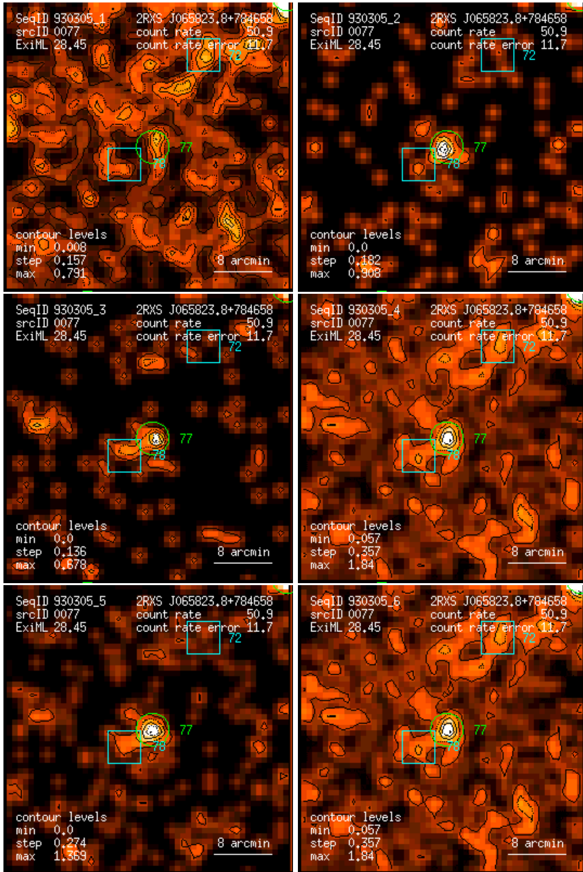
Figure 77: RASS 930305: detection 0077: band rate images, Gaussian filter: (1) PSPC channels 11 – 41, (2) 52 – 90, (3) 91 – 201, (4) 11 – 235, (5) 52 – 201, (6) 11 – 201. Broad band rates in counts/ks. Band rate contour levels in counts/ks/arcmin 2 .
