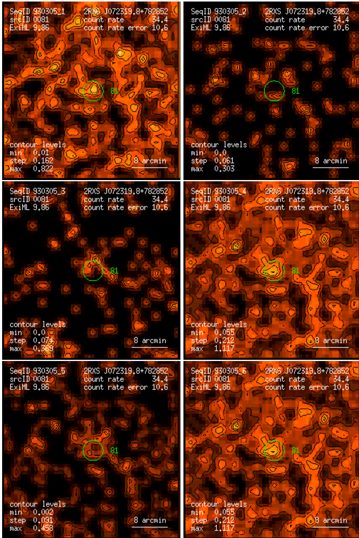
Figure 81: RASS 930305: detection 0081: band rate images, Gaussian filter: (1) PSPC channels 11 – 41, (2) 52 – 90, (3) 91 – 201, (4) 11 – 235, (5) 52 – 201, (6) 11 – 201. Broad band rates in counts/ks. Band rate contour levels in counts/ks/arcmin 2 .
