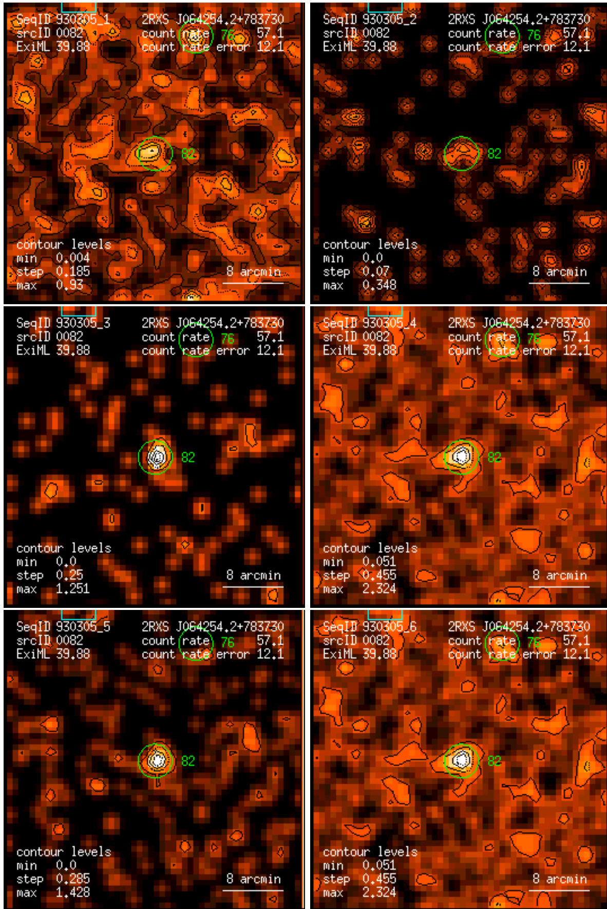
Figure 82: RASS 930305: detection 0082: band rate images, Gaussian filter: (1) PSPC channels 11 – 41, (2) 52 – 90, (3) 91 – 201, (4) 11 – 235, (5) 52 – 201, (6) 11 – 201. Broad band rates in counts/ks. Band rate contour levels in counts/ks/arcmin 2 .
