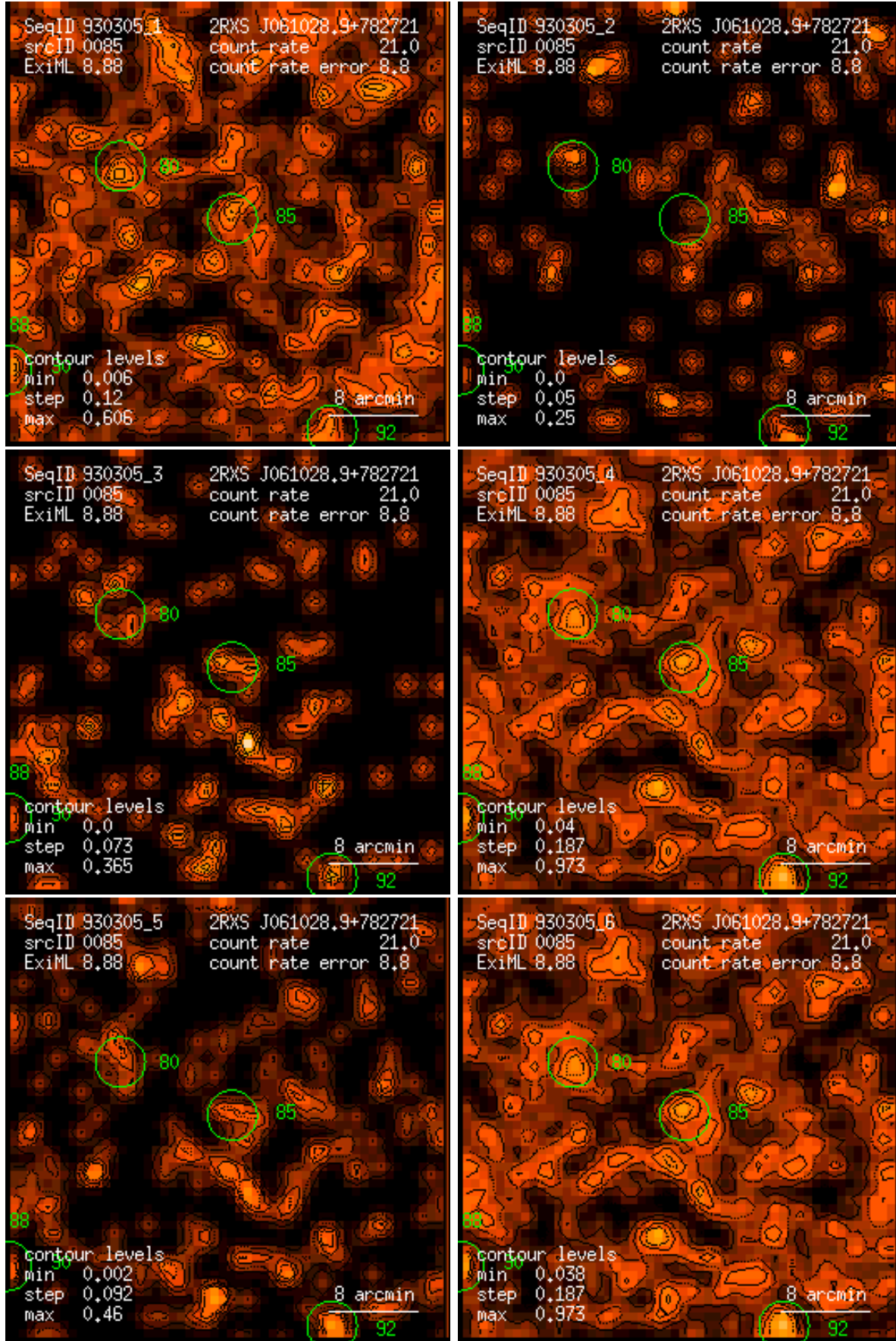
Figure 85: RASS 930305: detection 0085: band rate images, Gaussian filter: (1) PSPC channels 11 – 41, (2) 52 – 90, (3) 91 – 201, (4) 11 – 235, (5) 52 – 201, (6) 11 – 201. Broad band rates in counts/ks. Band rate contour levels in counts/ks/arcmin 2 .
