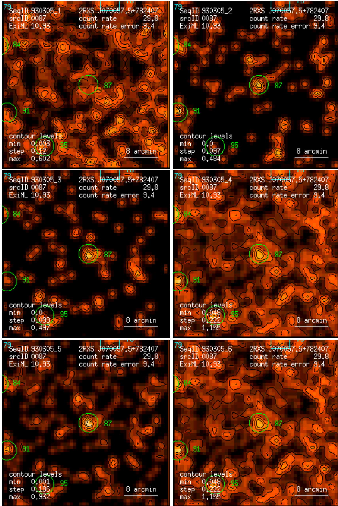
Figure 87: RASS 930305: detection 0087: band rate images, Gaussian filter: (1) PSPC channels 11 – 41, (2) 52 – 90, (3) 91 – 201, (4) 11 – 235, (5) 52 – 201, (6) 11 – 201. Broad band rates in counts/ks. Band rate contour levels in counts/ks/arcmin 2 .
