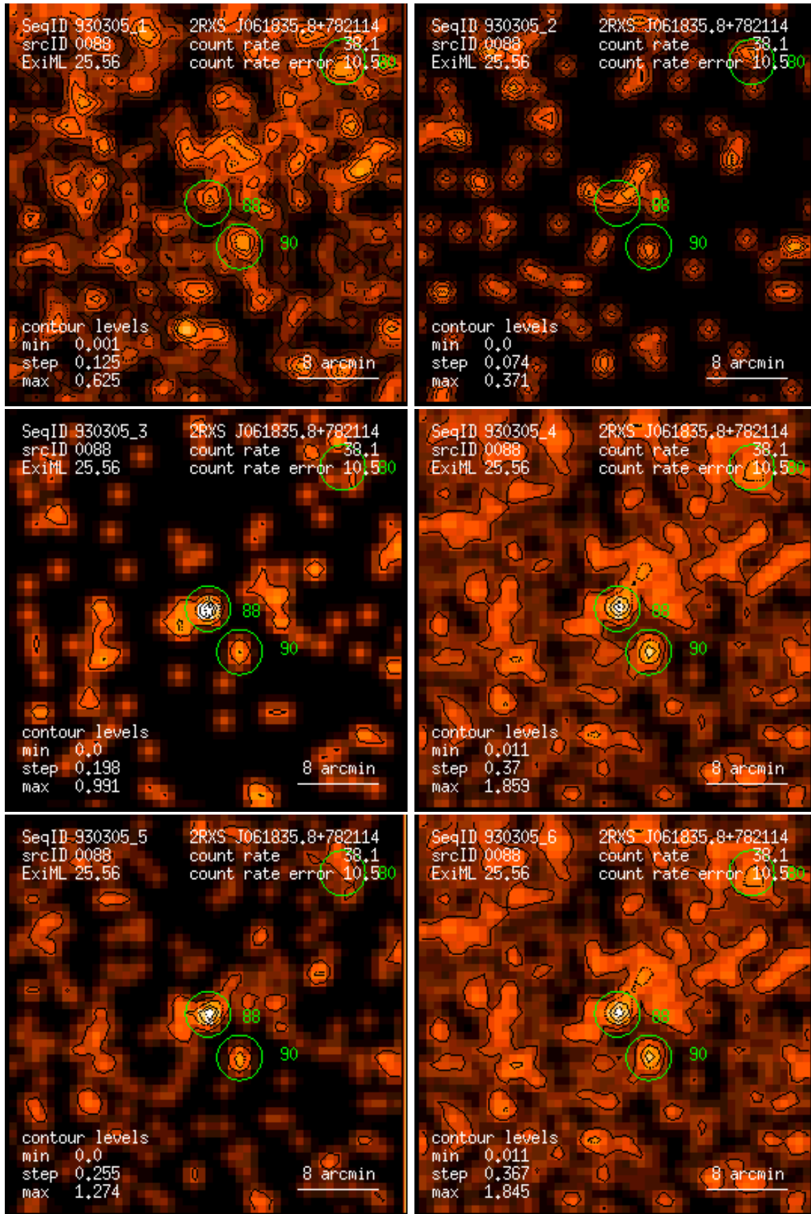
Figure 88: RASS 930305: detection 0088: band rate images, Gaussian filter: (1) PSPC channels 11 – 41, (2) 52 – 90, (3) 91 – 201, (4) 11 – 235, (5) 52 – 201, (6) 11 – 201. Broad band rates in counts/ks. Band rate contour levels in counts/ks/arcmin 2 .
