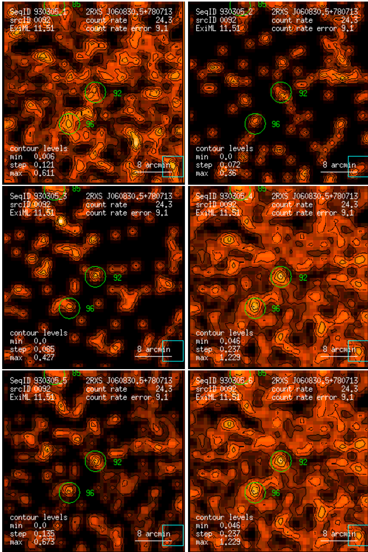
Figure 92: RASS 930305: detection 0092: band rate images, Gaussian filter: (1) PSPC channels 11 – 41, (2) 52 – 90, (3) 91 – 201, (4) 11 – 235, (5) 52 – 201, (6) 11 – 201. Broad band rates in counts/ks. Band rate contour levels in counts/ks/arcmin 2 .
