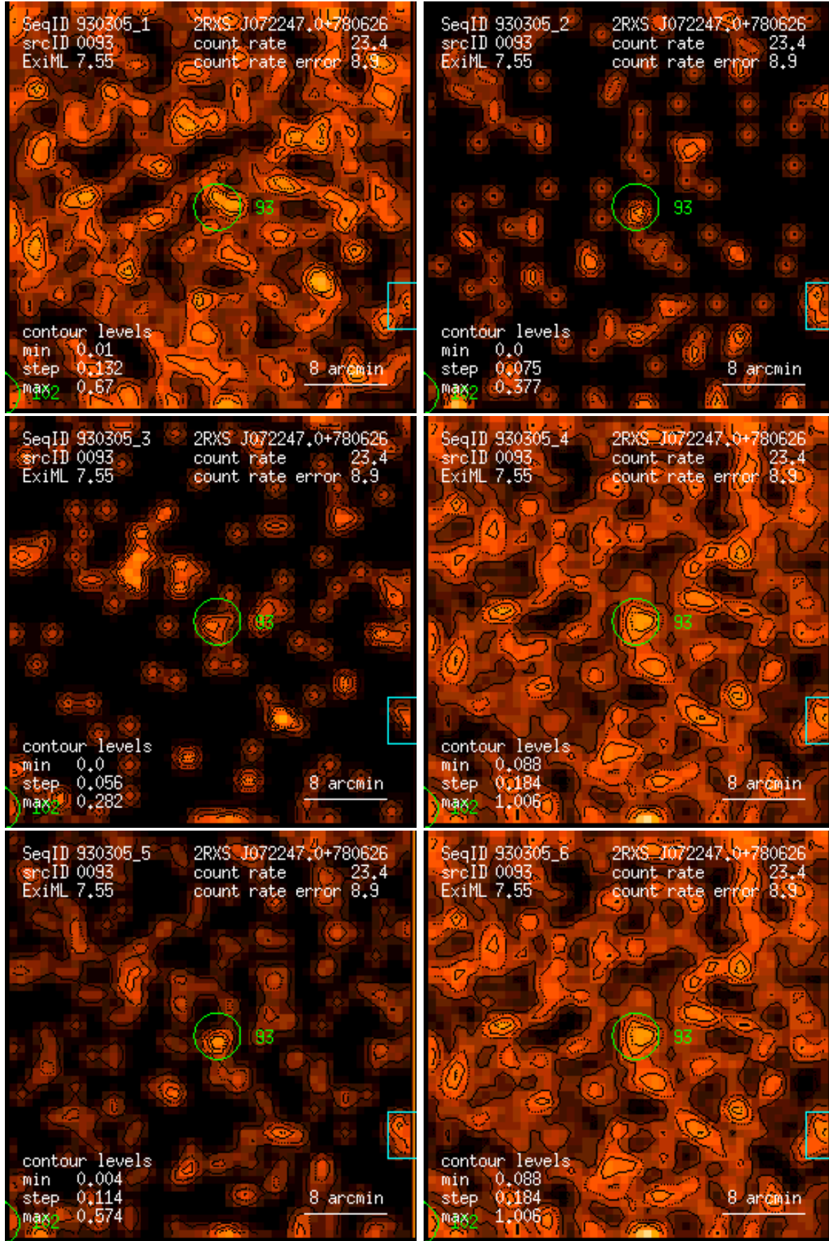
Figure 93: RASS 930305: detection 0093: band rate images, Gaussian filter: (1) PSPC channels 11 – 41, (2) 52 – 90, (3) 91 – 201, (4) 11 – 235, (5) 52 – 201, (6) 11 – 201. Broad band rates in counts/ks. Band rate contour levels in counts/ks/arcmin 2 .
