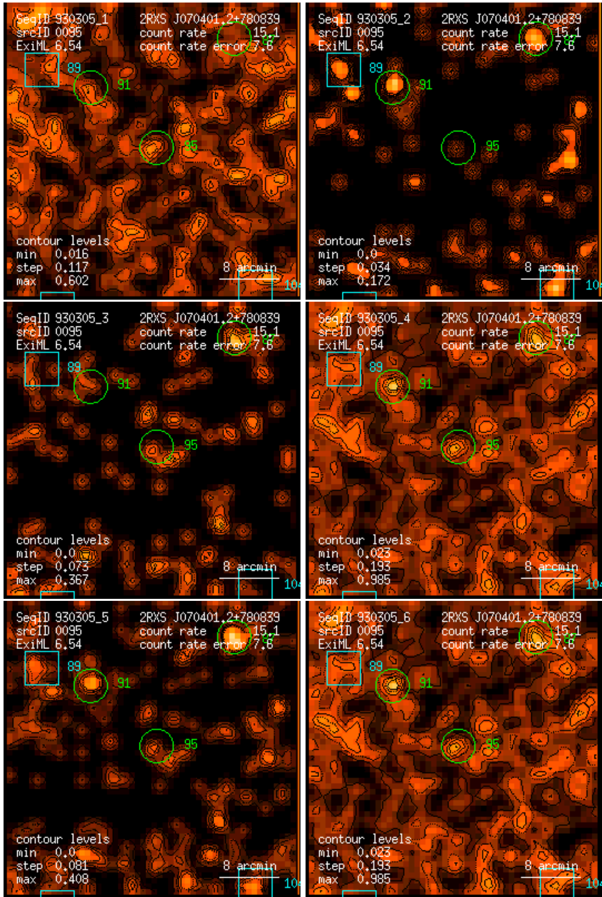
Figure 95: RASS 930305: detection 0095: band rate images, Gaussian filter: (1) PSPC channels 11 – 41, (2) 52 – 90, (3) 91 – 201, (4) 11 – 235, (5) 52 – 201, (6) 11 – 201. Broad band rates in counts/ks. Band rate contour levels in counts/ks/arcmin 2 .
