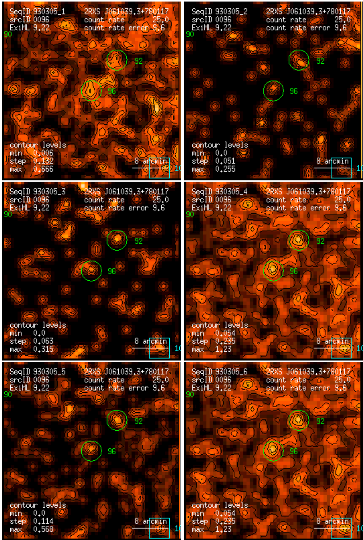
Figure 96: RASS 930305: detection 0096: band rate images, Gaussian filter: (1) PSPC channels 11 – 41, (2) 52 – 90, (3) 91 – 201, (4) 11 – 235, (5) 52 – 201, (6) 11 – 201. Broad band rates in counts/ks. Band rate contour levels in counts/ks/arcmin 2 .
