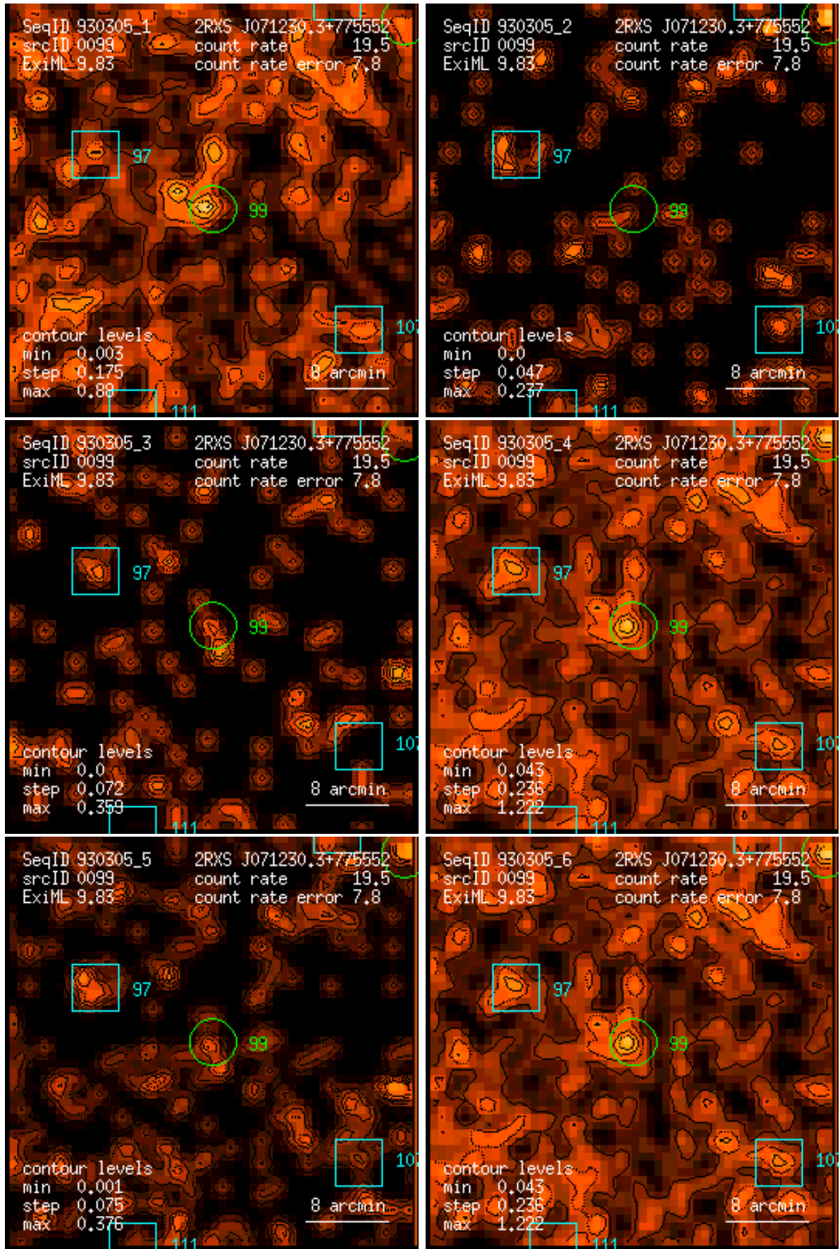
Figure 99: RASS 930305: detection 0099: band rate images, Gaussian filter: (1) PSPC channels 11 – 41, (2) 52 – 90, (3) 91 – 201, (4) 11 – 235, (5) 52 – 201, (6) 11 – 201. Broad band rates in counts/ks. Band rate contour levels in counts/ks/arcmin 2 .
