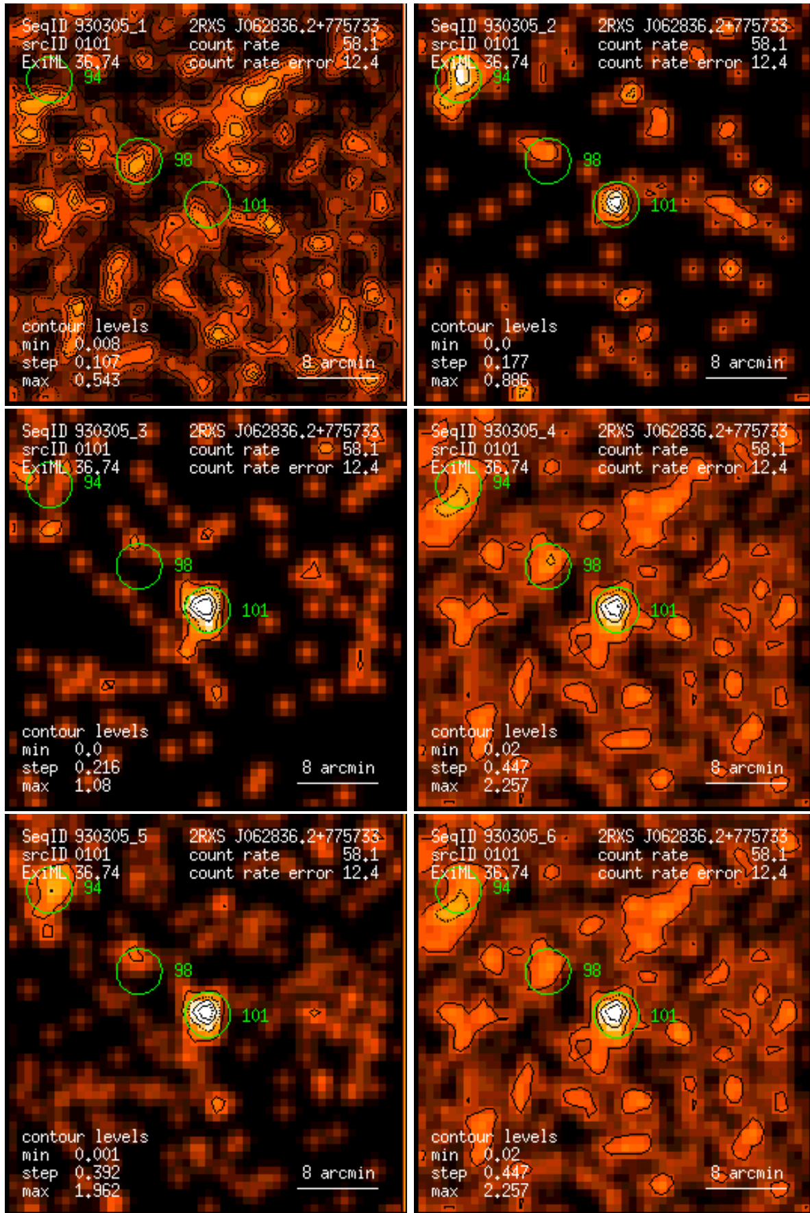
Figure 101: RASS 930305: detection 0101: band rate images, Gaussian filter: (1) PSPC channels 11 – 41, (2) 52 – 90, (3) 91 – 201, (4) 11 – 235, (5) 52 – 201, (6) 11 – 201. Broad band rates in counts/ks. Band rate contour levels in counts/ks/arcmin 2 .
