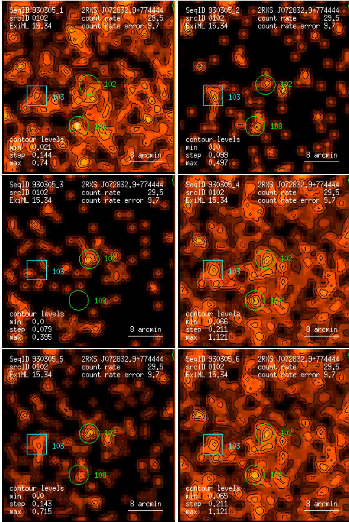
Figure 102: RASS 930305: detection 0102: band rate images, Gaussian filter: (1) PSPC channels 11 – 41, (2) 52 – 90, (3) 91 – 201, (4) 11 – 235, (5) 52 – 201, (6) 11 – 201. Broad band rates in counts/ks. Band rate contour levels in counts/ks/arcmin 2 .
