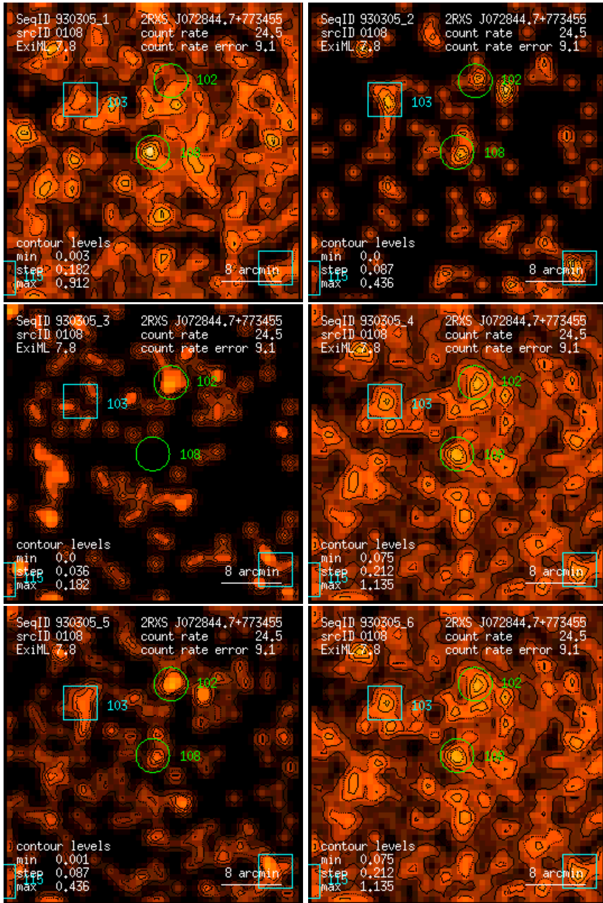
Figure 108: RASS 930305: detection 0108: band rate images, Gaussian filter: (1) PSPC channels 11 – 41, (2) 52 – 90, (3) 91 – 201, (4) 11 – 235, (5) 52 – 201, (6) 11 – 201. Broad band rates in counts/ks. Band rate contour levels in counts/ks/arcmin 2 .
