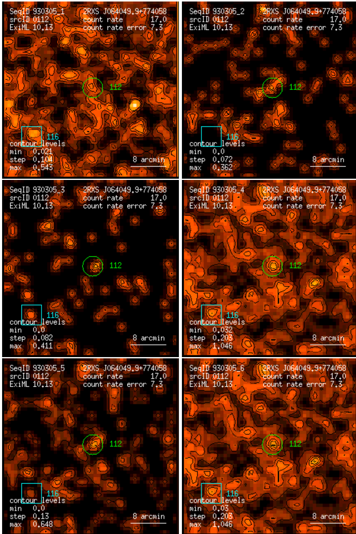
Figure 112: RASS 930305: detection 0112: band rate images, Gaussian filter: (1) PSPC channels 11 – 41, (2) 52 – 90, (3) 91 – 201, (4) 11 – 235, (5) 52 – 201, (6) 11 – 201. Broad band rates in counts/ks. Band rate contour levels in counts/ks/arcmin 2 .
