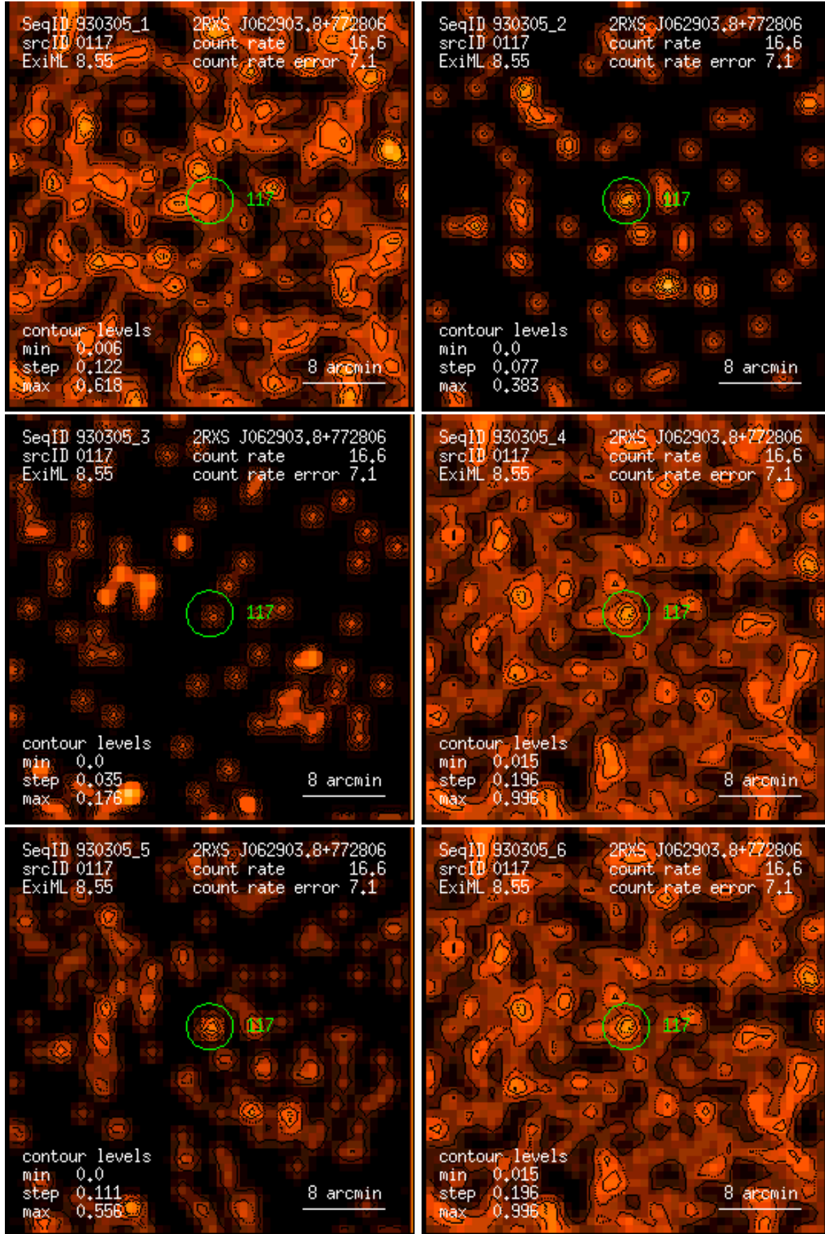
Figure 117: RASS 930305: detection 0117: band rate images, Gaussian filter: (1) PSPC channels 11 – 41, (2) 52 – 90, (3) 91 – 201, (4) 11 – 235, (5) 52 – 201, (6) 11 – 201. Broad band rates in counts/ks. Band rate contour levels in counts/ks/arcmin 2 .
