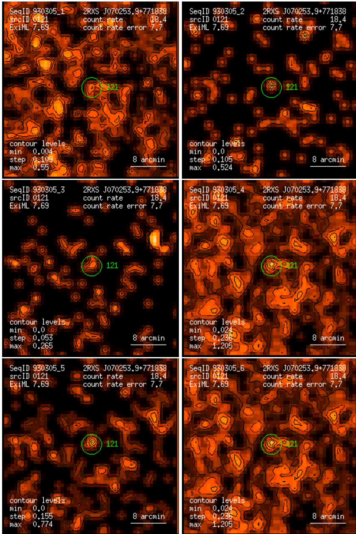
Figure 121: RASS 930305: detection 0121: band rate images, Gaussian filter: (1) PSPC channels 11 – 41, (2) 52 – 90, (3) 91 – 201, (4) 11 – 235, (5) 52 – 201, (6) 11 – 201. Broad band rates in counts/ks. Band rate contour levels in counts/ks/arcmin 2 .
