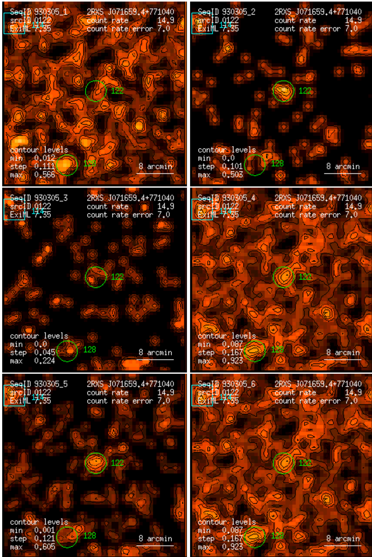
Figure 122: RASS 930305: detection 0122: band rate images, Gaussian filter: (1) PSPC channels 11 – 41, (2) 52 – 90, (3) 91 – 201, (4) 11 – 235, (5) 52 – 201, (6) 11 – 201. Broad band rates in counts/ks. Band rate contour levels in counts/ks/arcmin 2 .
