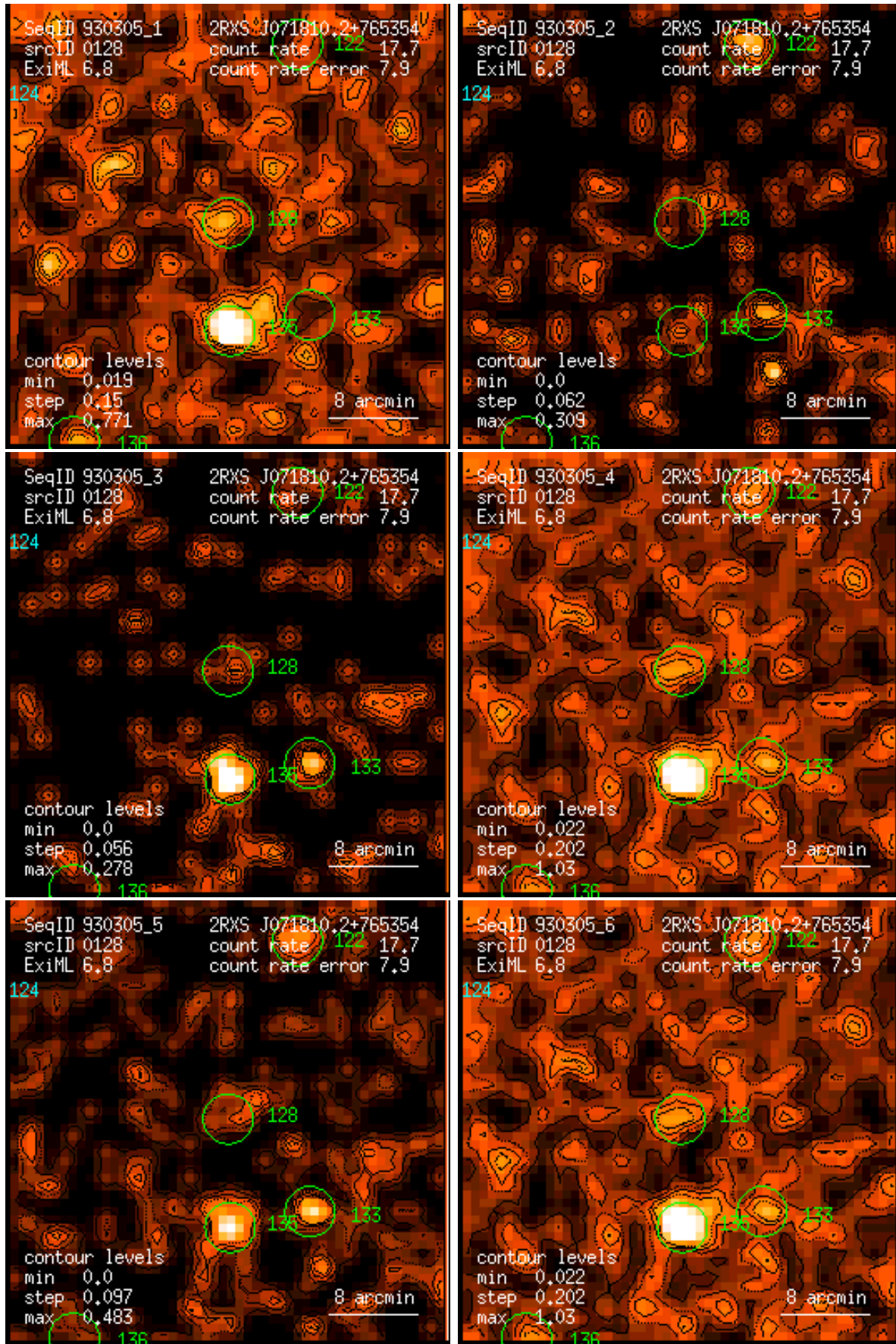
Figure 128: RASS 930305: detection 0128: band rate images, Gaussian filter: (1) PSPC channels 11 – 41, (2) 52 – 90, (3) 91 – 201, (4) 11 – 235, (5) 52 – 201, (6) 11 – 201. Broad band rates in counts/ks. Band rate contour levels in counts/ks/arcmin 2 .
