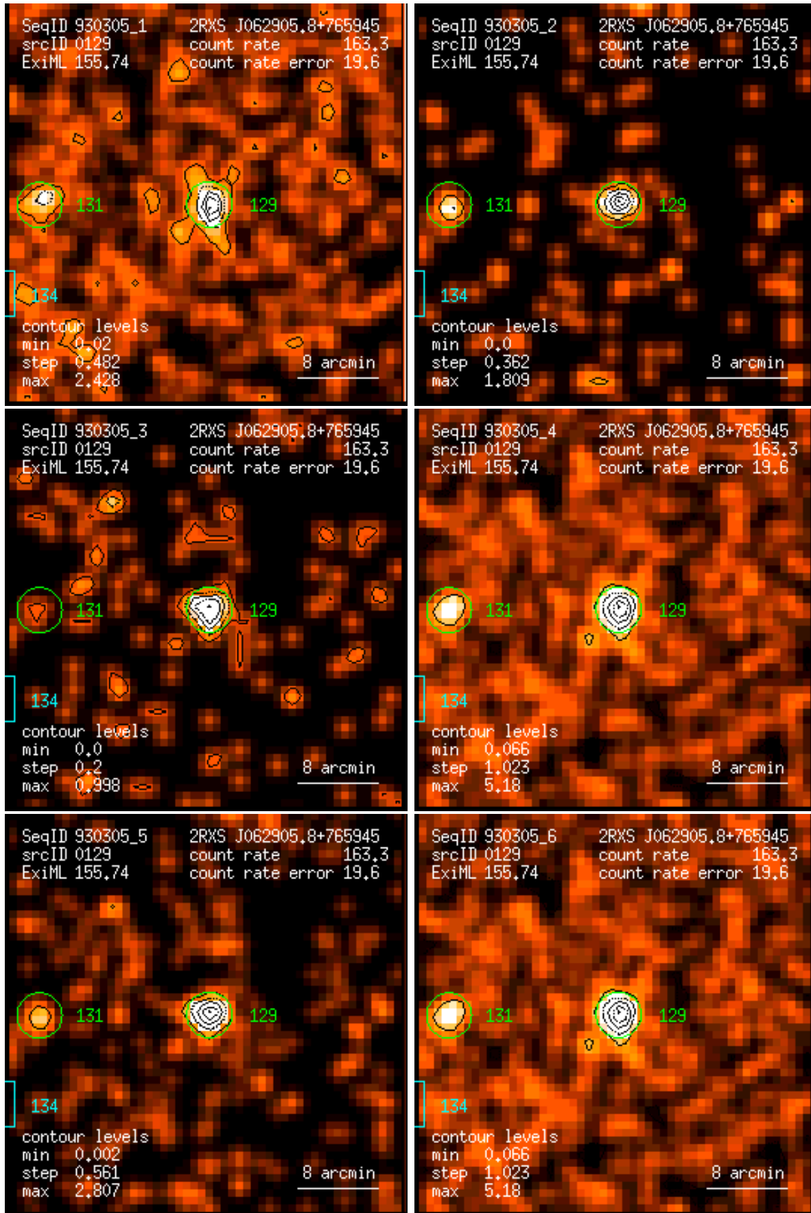
Figure 129: RASS 930305: detection 0129: band rate images, Gaussian filter: (1) PSPC channels 11 – 41, (2) 52 – 90, (3) 91 – 201, (4) 11 – 235, (5) 52 – 201, (6) 11 – 201. Broad band rates in counts/ks. Band rate contour levels in counts/ks/arcmin 2 .
