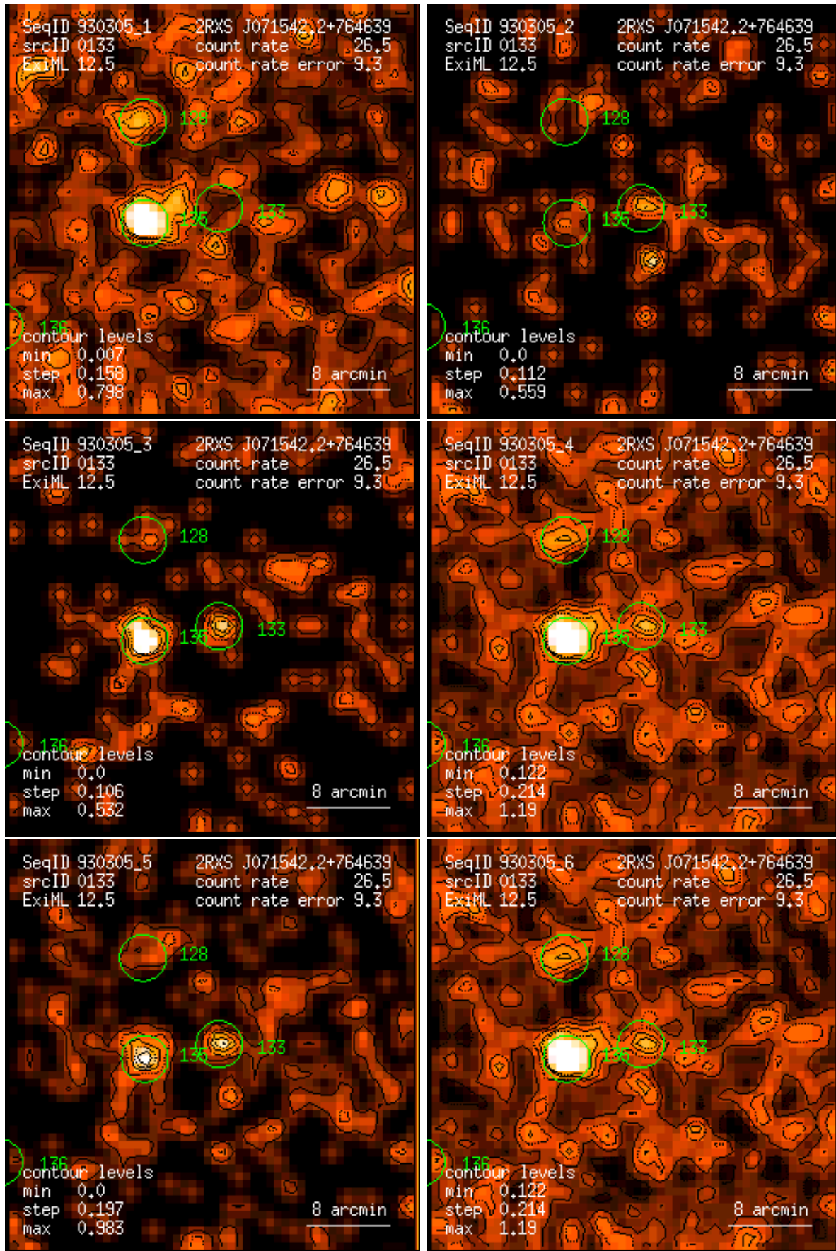
Figure 133: RASS 930305: detection 0133: band rate images, Gaussian filter: (1) PSPC channels 11 – 41, (2) 52 – 90, (3) 91 – 201, (4) 11 – 235, (5) 52 – 201, (6) 11 – 201. Broad band rates in counts/ks. Band rate contour levels in counts/ks/arcmin 2 .
