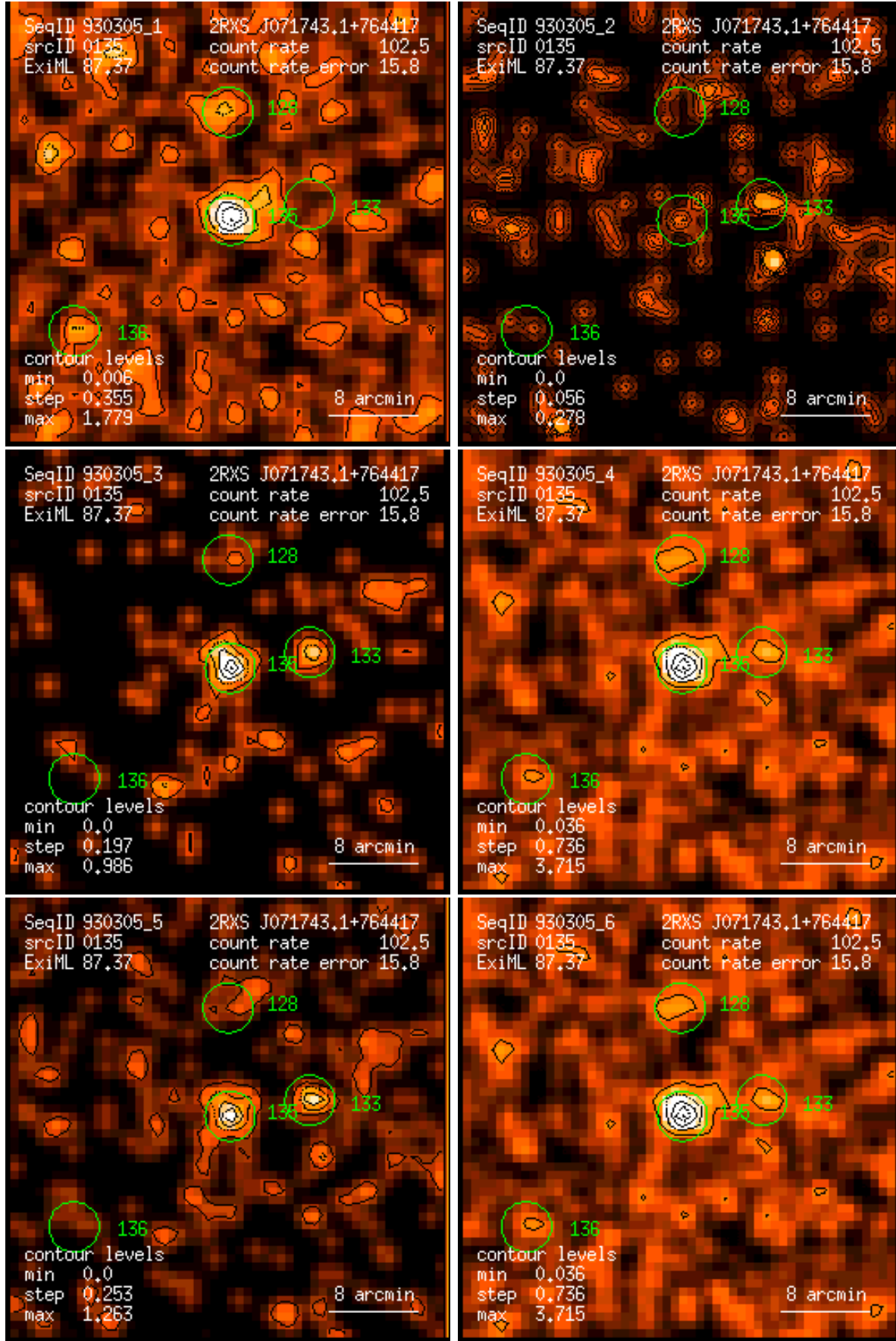
Figure 135: RASS 930305: detection 0135: band rate images, Gaussian filter: (1) PSPC channels 11 – 41, (2) 52 – 90, (3) 91 – 201, (4) 11 – 235, (5) 52 – 201, (6) 11 – 201. Broad band rates in counts/ks. Band rate contour levels in counts/ks/arcmin 2 .
