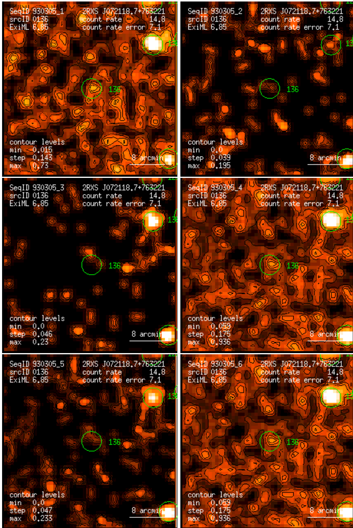
Figure 136: RASS 930305: detection 0136: band rate images, Gaussian filter: (1) PSPC channels 11 – 41, (2) 52 – 90, (3) 91 – 201, (4) 11 – 235, (5) 52 – 201, (6) 11 – 201. Broad band rates in counts/ks. Band rate contour levels in counts/ks/arcmin 2 .
