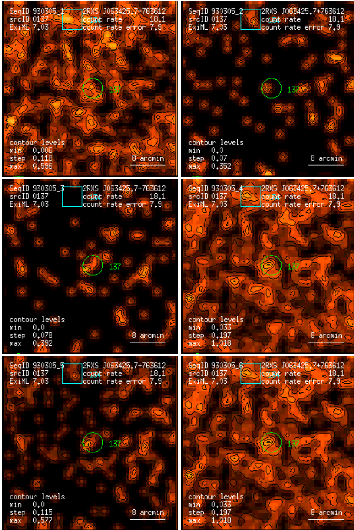
Figure 137: RASS 930305: detection 0137: band rate images, Gaussian filter: (1) PSPC channels 11 – 41, (2) 52 – 90, (3) 91 – 201, (4) 11 – 235, (5) 52 – 201, (6) 11 – 201. Broad band rates in counts/ks. Band rate contour levels in counts/ks/arcmin 2 .
