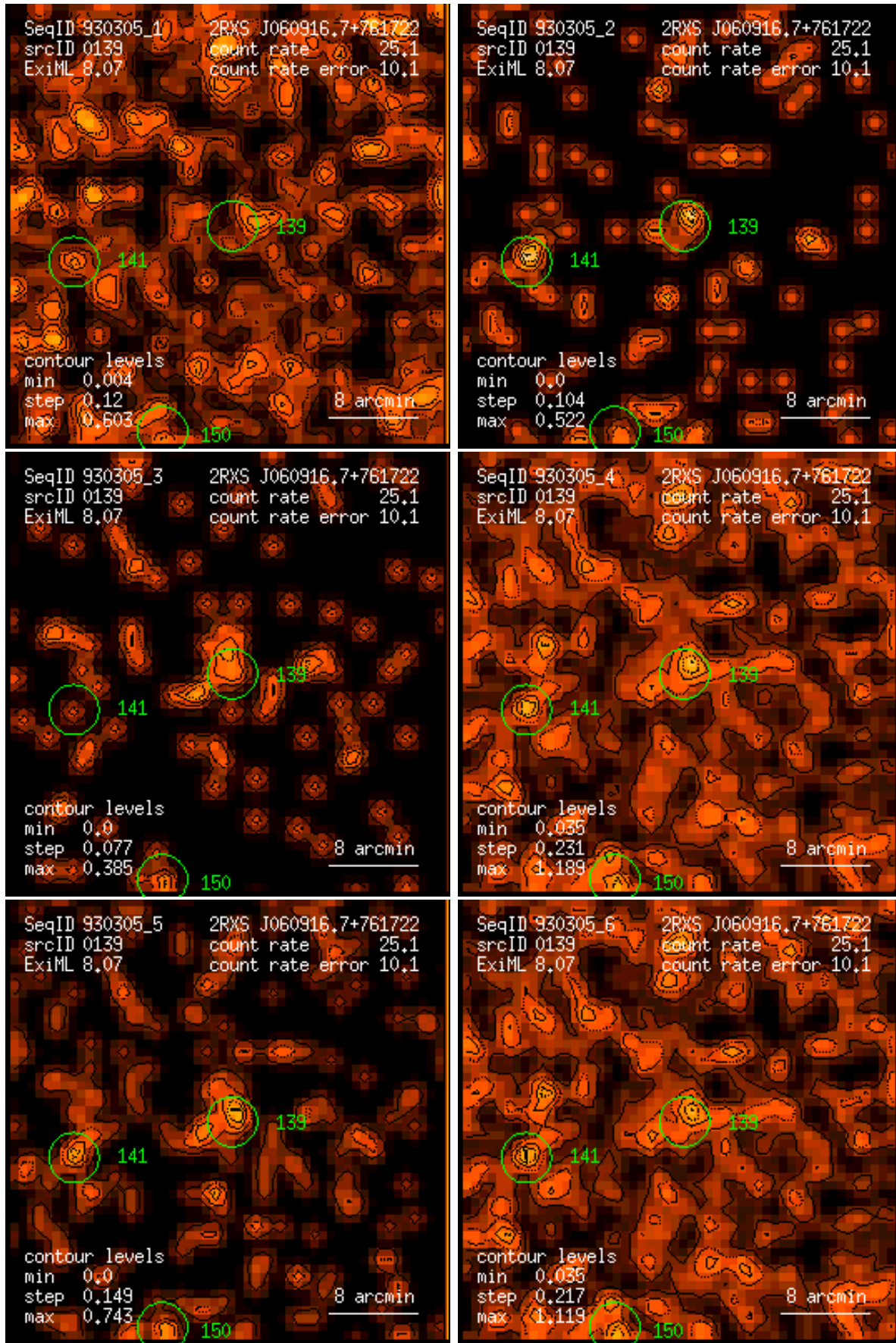
Figure 139: RASS 930305: detection 0139: band rate images, Gaussian filter: (1) PSPC channels 11 – 41, (2) 52 – 90, (3) 91 – 201, (4) 11 – 235, (5) 52 – 201, (6) 11 – 201. Broad band rates in counts/ks. Band rate contour levels in counts/ks/arcmin 2 .
