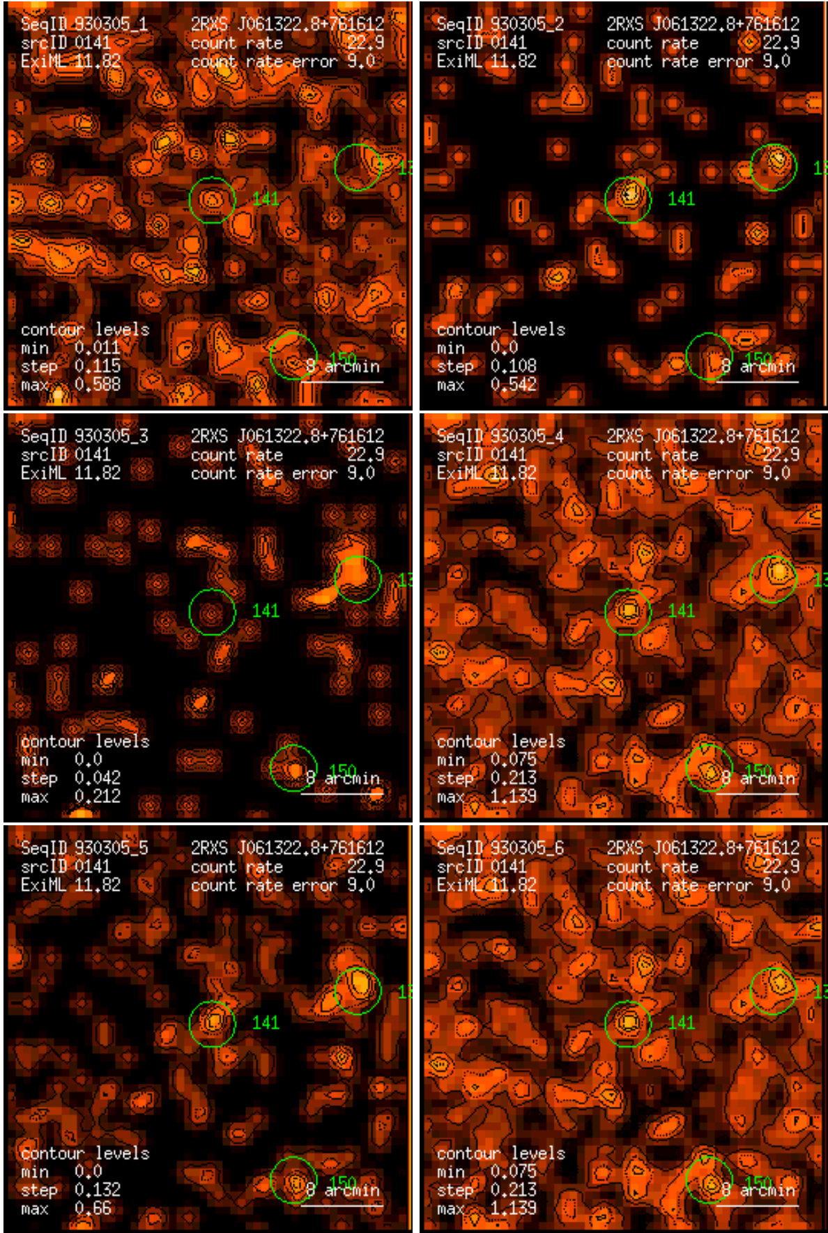
Figure 141: RASS 930305: detection 0141: band rate images, Gaussian filter: (1) PSPC channels 11 – 41, (2) 52 – 90, (3) 91 – 201, (4) 11 – 235, (5) 52 – 201, (6) 11 – 201. Broad band rates in counts/ks. Band rate contour levels in counts/ks/arcmin 2 .
