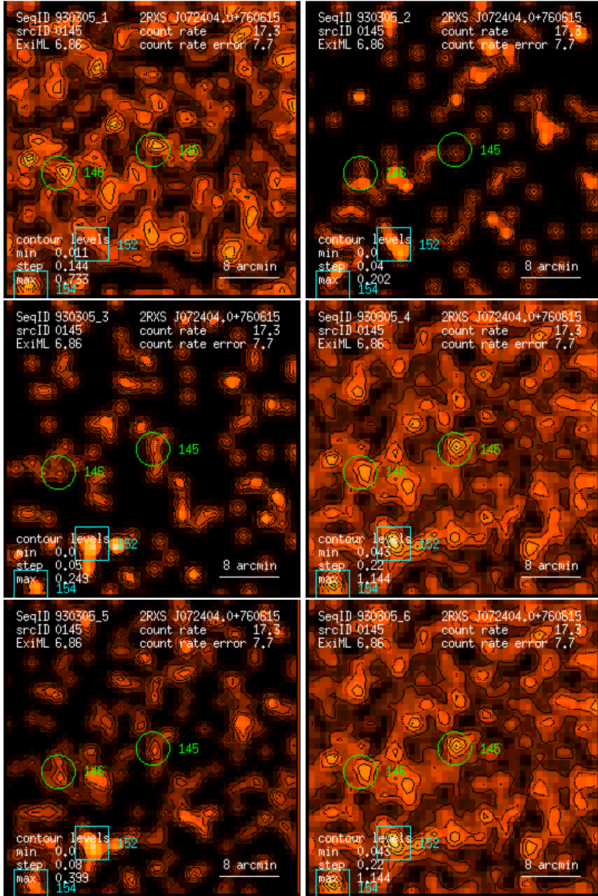
Figure 145: RASS 930305: detection 0145: band rate images, Gaussian filter: (1) PSPC channels 11 – 41, (2) 52 – 90, (3) 91 – 201, (4) 11 – 235, (5) 52 – 201, (6) 11 – 201. Broad band rates in counts/ks. Band rate contour levels in counts/ks/arcmin 2 .
