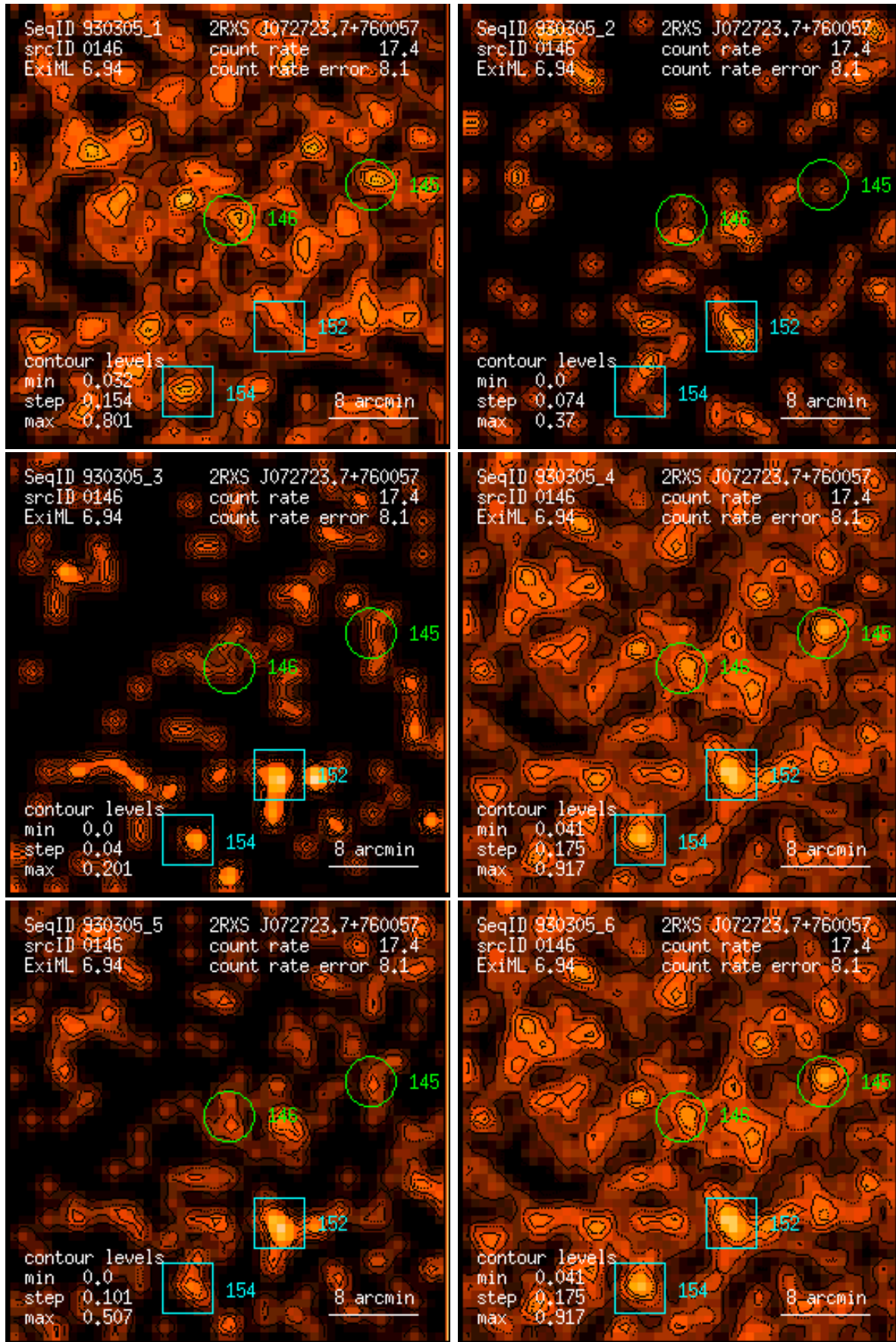
Figure 146: RASS 930305: detection 0146: band rate images, Gaussian filter: (1) PSPC channels 11 – 41, (2) 52 – 90, (3) 91 – 201, (4) 11 – 235, (5) 52 – 201, (6) 11 – 201. Broad band rates in counts/ks. Band rate contour levels in counts/ks/arcmin 2 .
