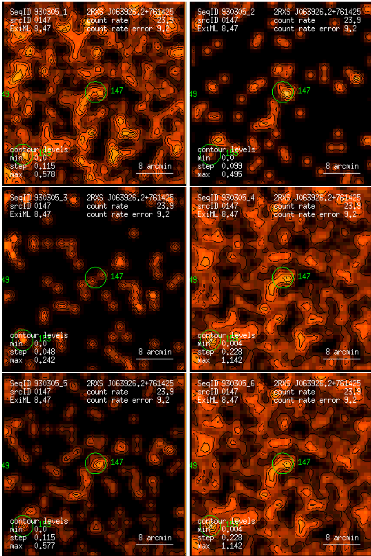
Figure 147: RASS 930305: detection 0147: band rate images, Gaussian filter: (1) PSPC channels 11 – 41, (2) 52 – 90, (3) 91 – 201, (4) 11 – 235, (5) 52 – 201, (6) 11 – 201. Broad band rates in counts/ks. Band rate contour levels in counts/ks/arcmin 2 .
