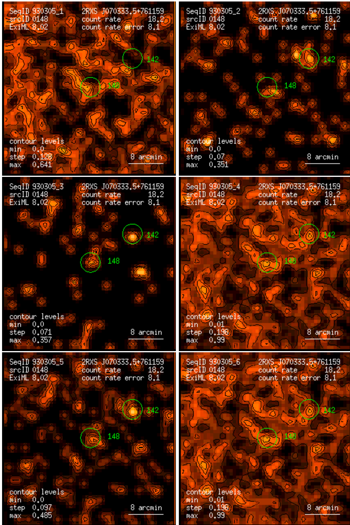
Figure 148: RASS 930305: detection 0148: band rate images, Gaussian filter: (1) PSPC channels 11 – 41, (2) 52 – 90, (3) 91 – 201, (4) 11 – 235, (5) 52 – 201, (6) 11 – 201. Broad band rates in counts/ks. Band rate contour levels in counts/ks/arcmin 2 .
