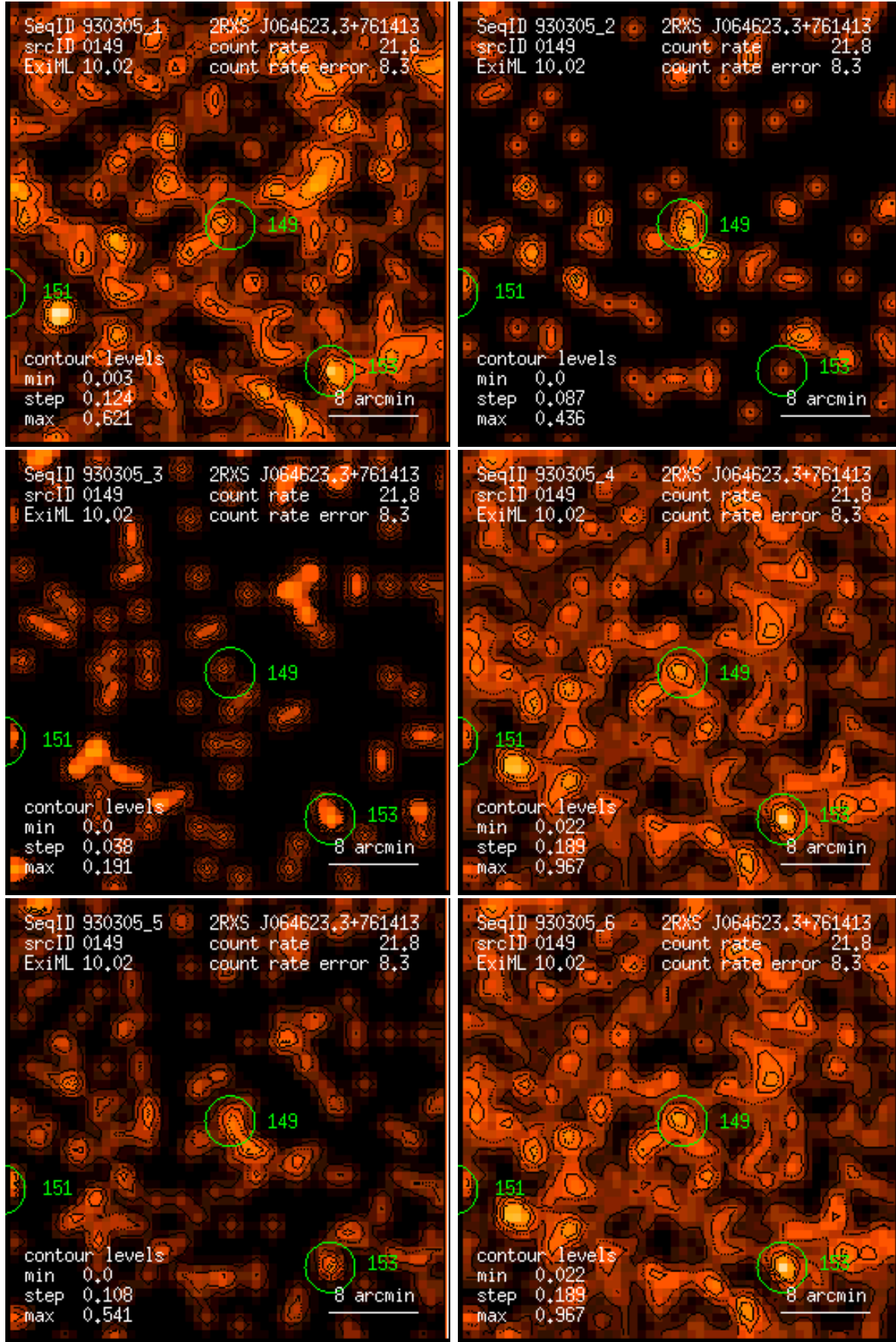
Figure 149: RASS 930305: detection 0149: band rate images, Gaussian filter: (1) PSPC channels 11 – 41, (2) 52 – 90, (3) 91 – 201, (4) 11 – 235, (5) 52 – 201, (6) 11 – 201. Broad band rates in counts/ks. Band rate contour levels in counts/ks/arcmin 2 .
