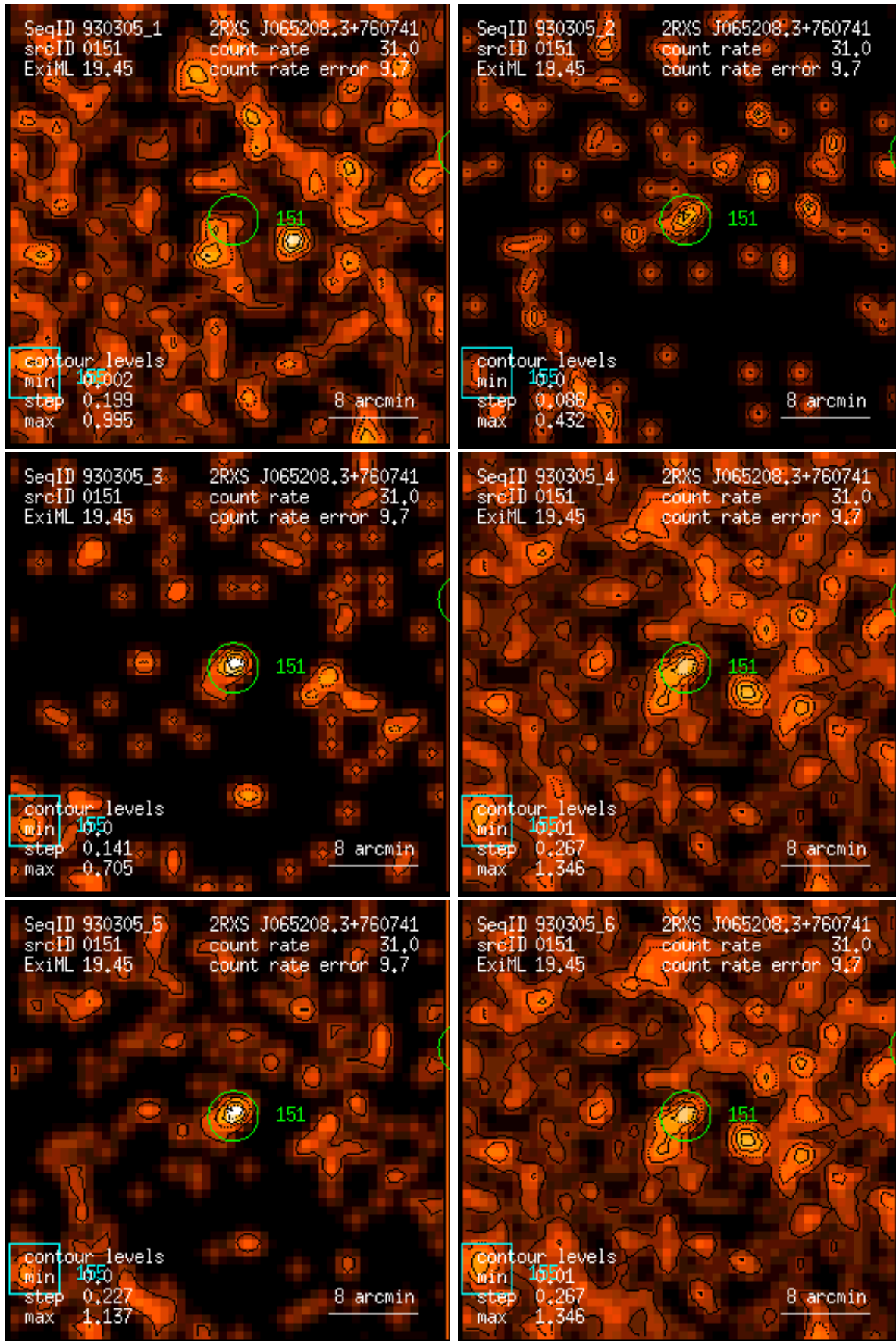
Figure 151: RASS 930305: detection 0151: band rate images, Gaussian filter: (1) PSPC channels 11 – 41, (2) 52 – 90, (3) 91 – 201, (4) 11 – 235, (5) 52 – 201, (6) 11 – 201. Broad band rates in counts/ks. Band rate contour levels in counts/ks/arcmin 2 .
