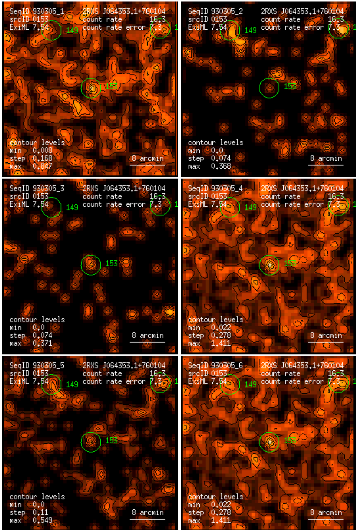
Figure 153: RASS 930305: detection 0153: band rate images, Gaussian filter: (1) PSPC channels 11 – 41, (2) 52 – 90, (3) 91 – 201, (4) 11 – 235, (5) 52 – 201, (6) 11 – 201. Broad band rates in counts/ks. Band rate contour levels in counts/ks/arcmin 2 .
