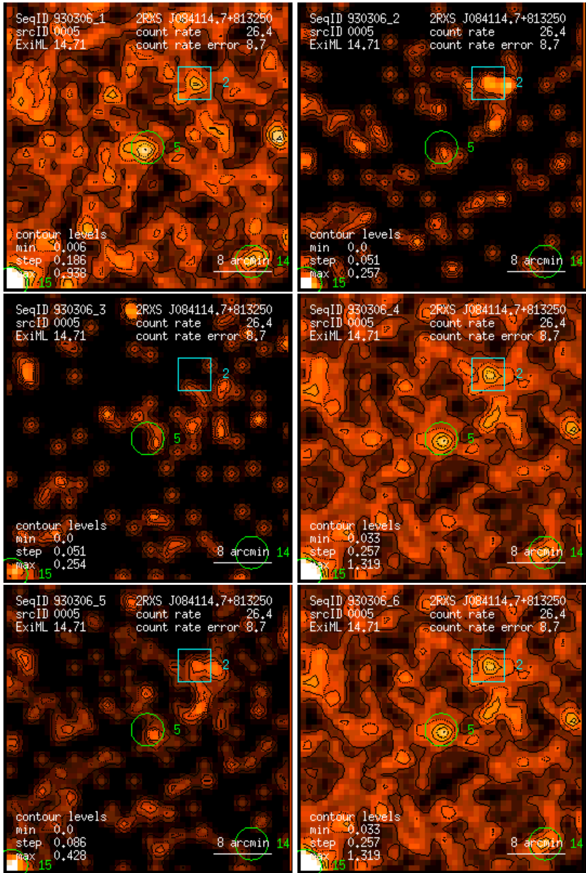
Figure 5: RASS 930306: detection 0005: band rate images, Gaussian filter: (1) PSPC channels 11 – 41, (2) 52 – 90, (3) 91 – 201, (4) 11 – 235, (5) 52 – 201, (6) 11 – 201. Broad band rates in counts/ks. Band rate contour levels in counts/ks/arcmin 2 .
