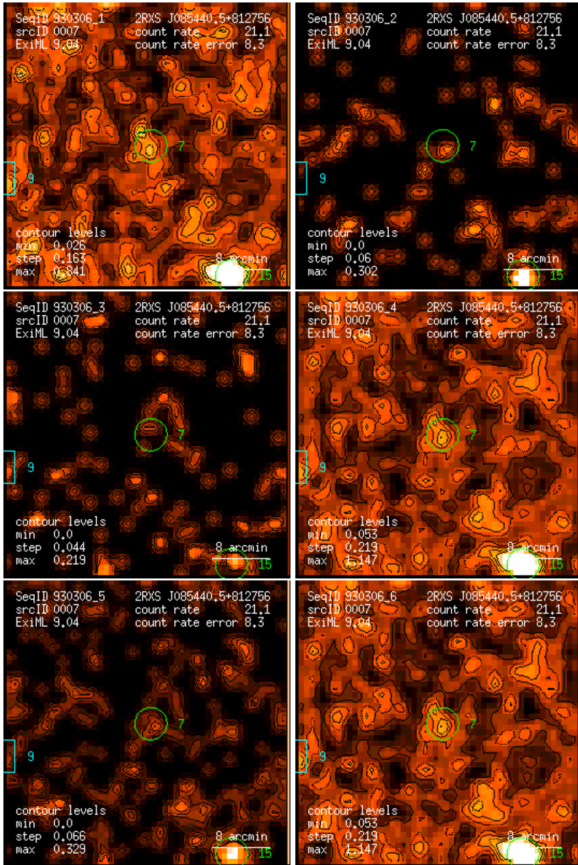
Figure 7: RASS 930306: detection 0007: band rate images, Gaussian filter: (1) PSPC channels 11 – 41, (2) 52 – 90, (3) 91 – 201, (4) 11 – 235, (5) 52 – 201, (6) 11 – 201. Broad band rates in counts/ks. Band rate contour levels in counts/ks/arcmin 2 .
